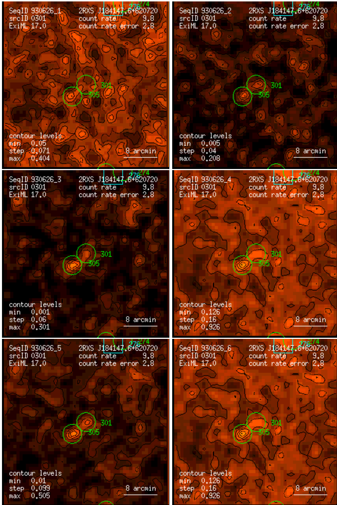
Figure 301: RASS 930626: detection 0301: band rate images, Gaussian filter: (1) PSPC channels 11 – 41, (2) 52 – 90, (3) 91 – 201, (4) 11 – 235, (5) 52 – 201, (6) 11 – 201. Broad band rates in counts/ks. Band rate contour levels in counts/ks/arcmin 2 .
