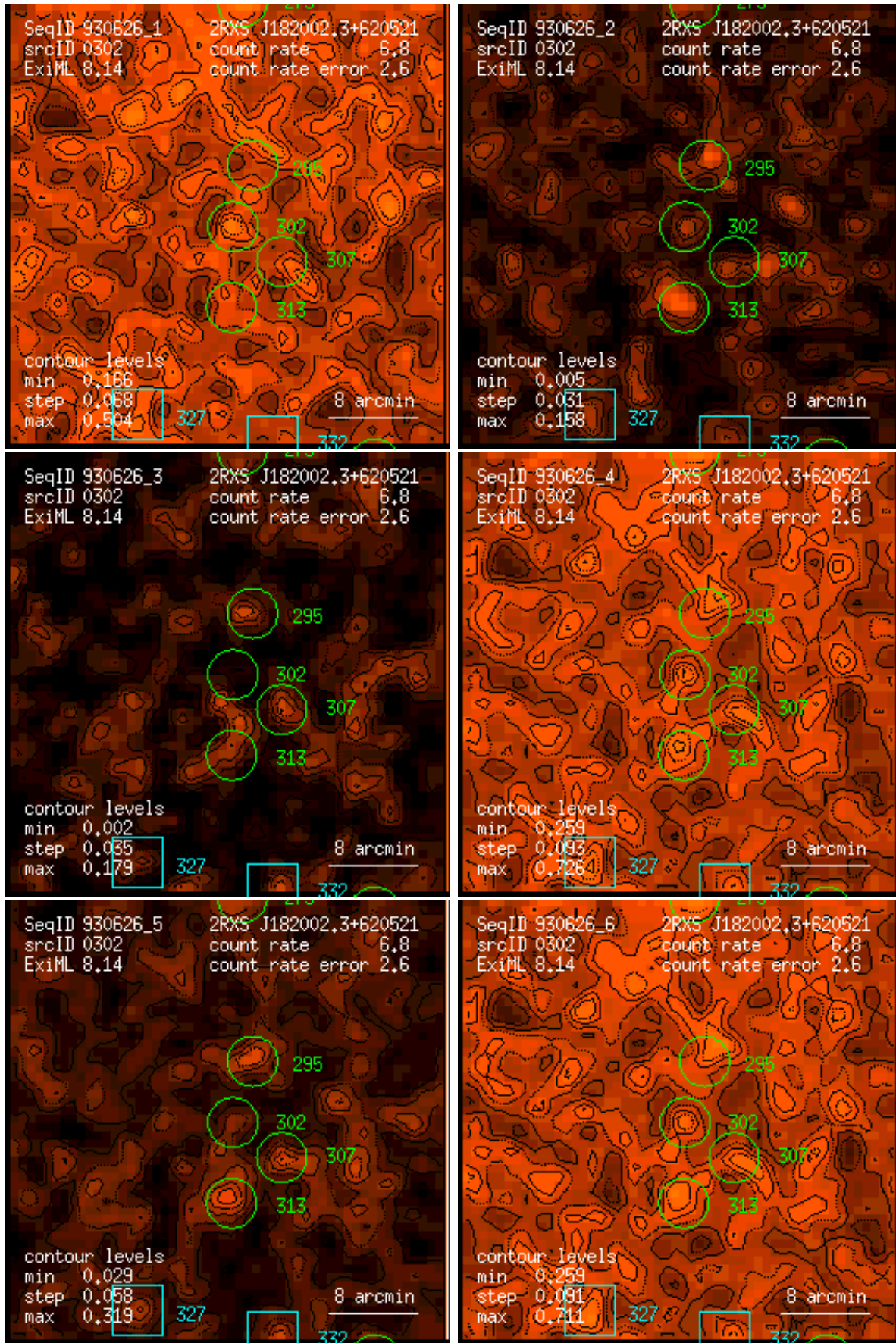
Figure 302: RASS 930626: detection 0302: band rate images, Gaussian filter: (1) PSPC channels 11 – 41, (2) 52 – 90, (3) 91 – 201, (4) 11 – 235, (5) 52 – 201, (6) 11 – 201. Broad band rates in counts/ks. Band rate contour levels in counts/ks/arcmin 2 .
