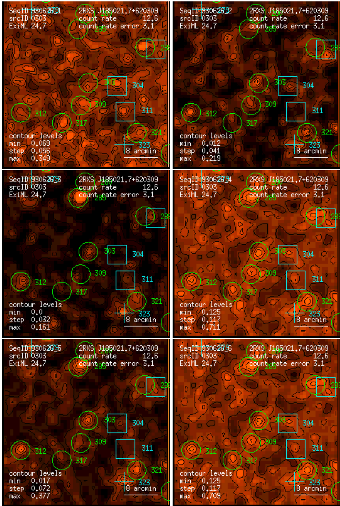
Figure 303: RASS 930626: detection 0303: band rate images, Gaussian filter: (1) PSPC channels 11 – 41, (2) 52 – 90, (3) 91 – 201, (4) 11 – 235, (5) 52 – 201, (6) 11 – 201. Broad band rates in counts/ks. Band rate contour levels in counts/ks/arcmin 2 .
