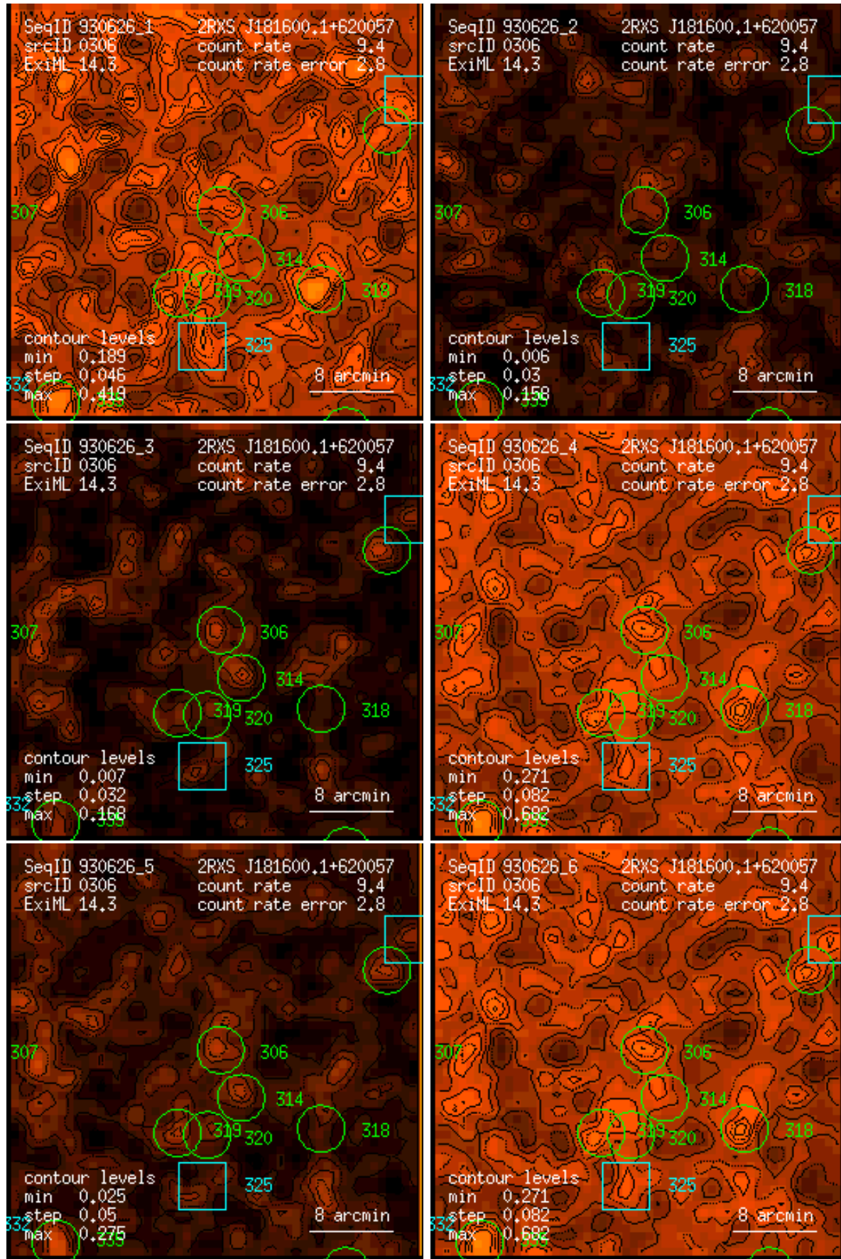
Figure 306: RASS 930626: detection 0306: band rate images, Gaussian filter: (1) PSPC channels 11 – 41, (2) 52 – 90, (3) 91 – 201, (4) 11 – 235, (5) 52 – 201, (6) 11 – 201. Broad band rates in counts/ks. Band rate contour levels in counts/ks/arcmin 2 .
