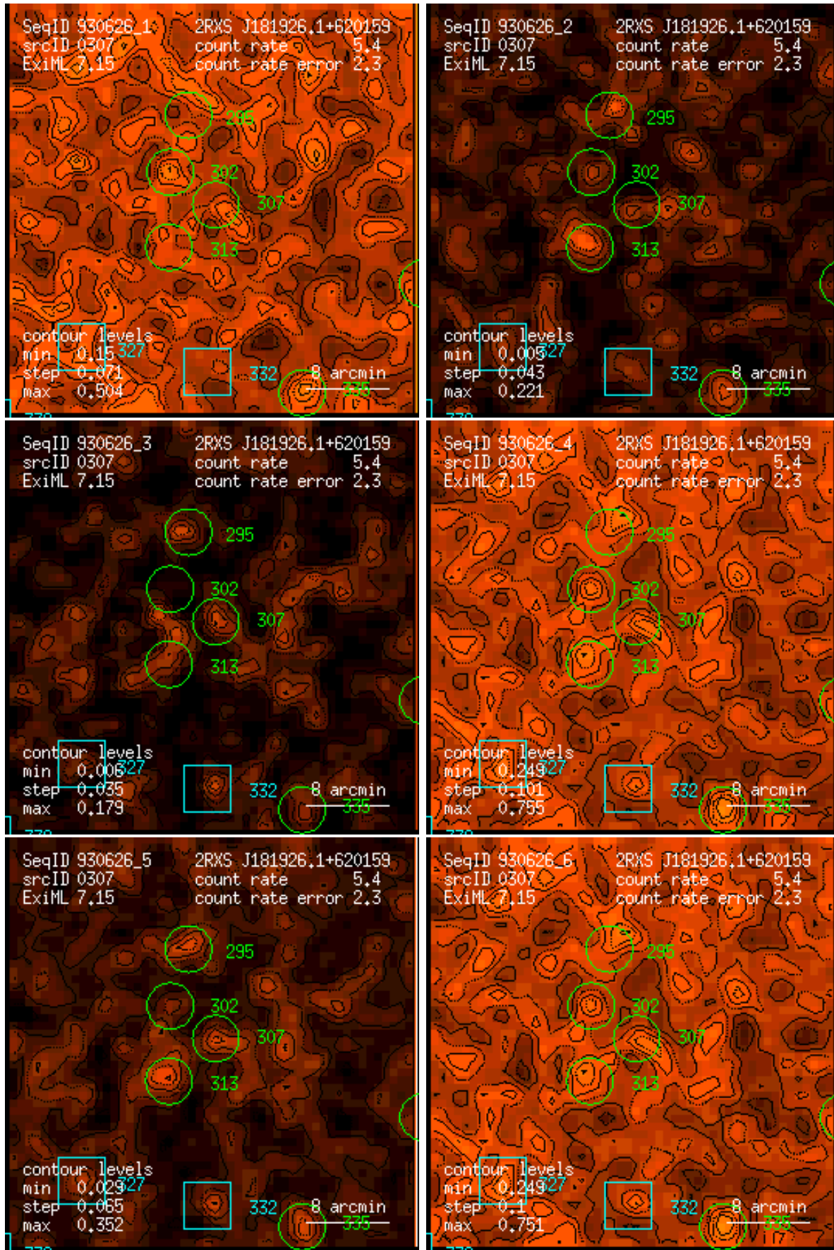
Figure 307: RASS 930626: detection 0307: band rate images, Gaussian filter: (1) PSPC channels 11 – 41, (2) 52 – 90, (3) 91 – 201, (4) 11 – 235, (5) 52 – 201, (6) 11 – 201. Broad band rates in counts/ks. Band rate contour levels in counts/ks/arcmin 2 .
