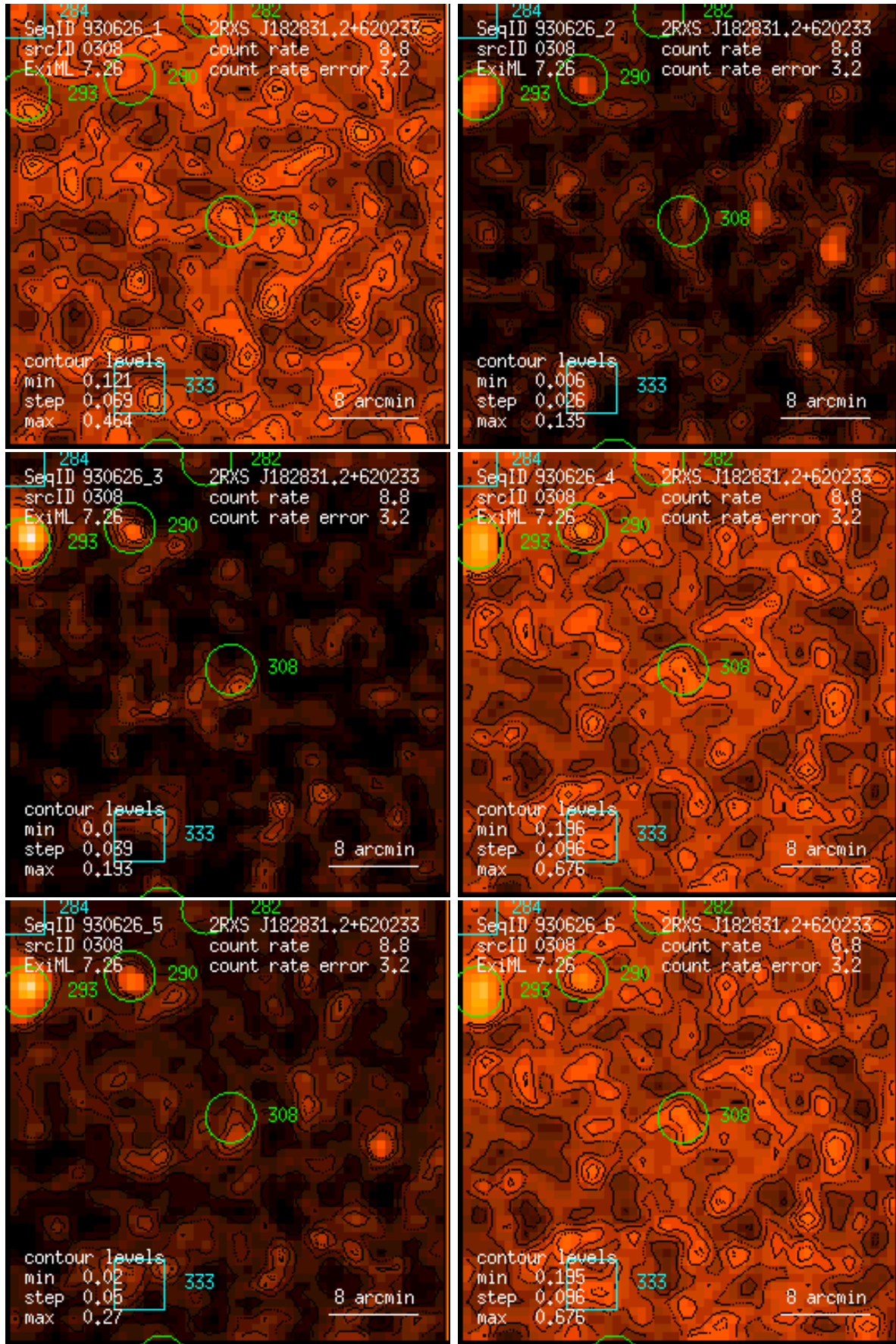
Figure 308: RASS 930626: detection 0308: band rate images, Gaussian filter: (1) PSPC channels 11 – 41, (2) 52 – 90, (3) 91 – 201, (4) 11 – 235, (5) 52 – 201, (6) 11 – 201. Broad band rates in counts/ks. Band rate contour levels in counts/ks/arcmin 2 .
