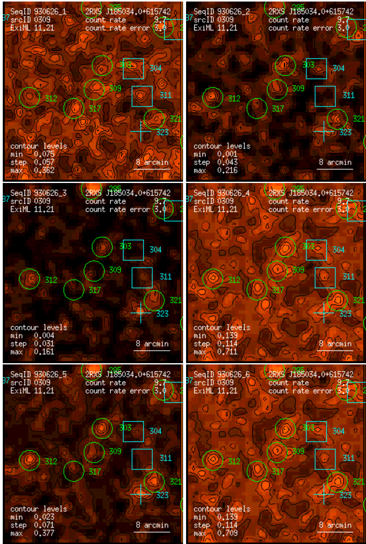
Figure 309: RASS 930626: detection 0309: band rate images, Gaussian filter: (1) PSPC channels 11 – 41, (2) 52 – 90, (3) 91 – 201, (4) 11 – 235, (5) 52 – 201, (6) 11 – 201. Broad band rates in counts/ks. Band rate contour levels in counts/ks/arcmin 2 .
