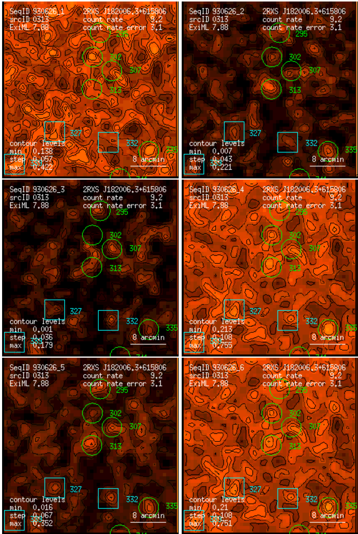
Figure 313: RASS 930626: detection 0313: band rate images, Gaussian filter: (1) PSPC channels 11 – 41, (2) 52 – 90, (3) 91 – 201, (4) 11 – 235, (5) 52 – 201, (6) 11 – 201. Broad band rates in counts/ks. Band rate contour levels in counts/ks/arcmin 2 .
