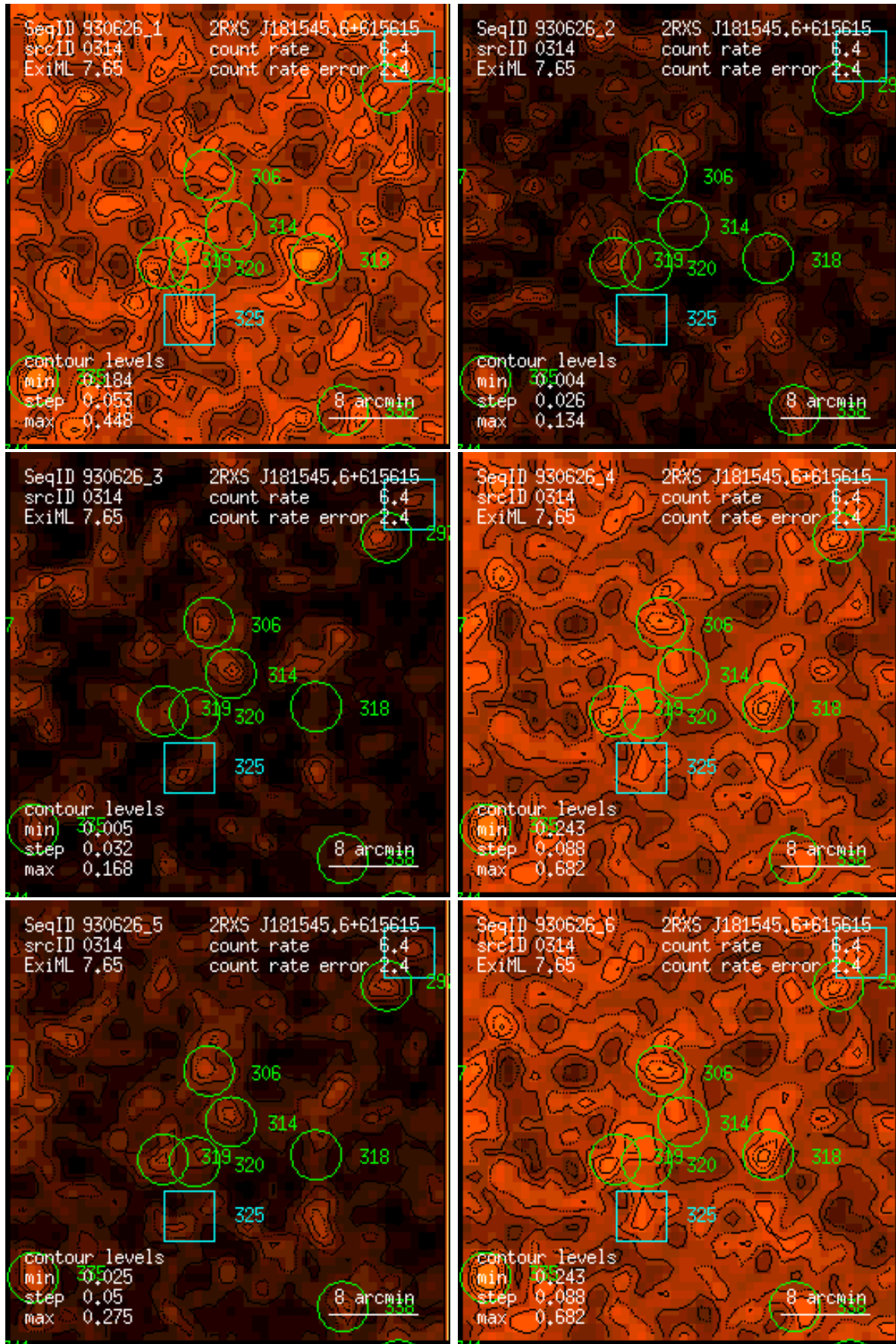
Figure 314: RASS 930626: detection 0314: band rate images, Gaussian filter: (1) PSPC channels 11 – 41, (2) 52 – 90, (3) 91 – 201, (4) 11 – 235, (5) 52 – 201, (6) 11 – 201. Broad band rates in counts/ks. Band rate contour levels in counts/ks/arcmin 2 .
