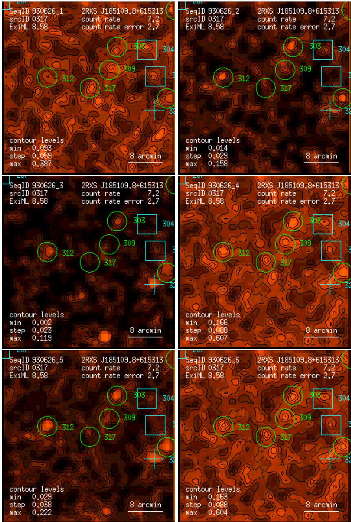
Figure 317: RASS 930626: detection 0317: band rate images, Gaussian filter: (1) PSPC channels 11 – 41, (2) 52 – 90, (3) 91 – 201, (4) 11 – 235, (5) 52 – 201, (6) 11 – 201. Broad band rates in counts/ks. Band rate contour levels in counts/ks/arcmin 2 .
