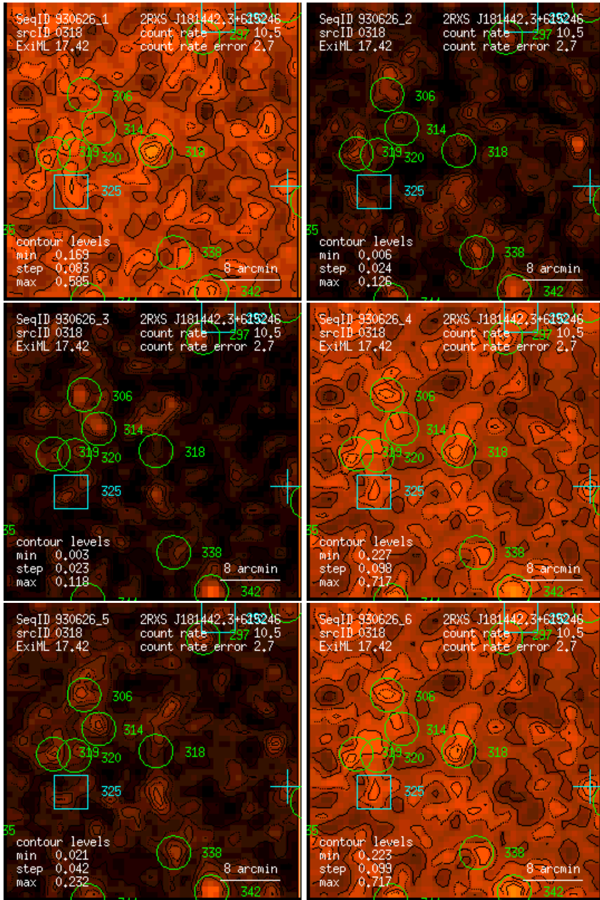
Figure 318: RASS 930626: detection 0318: band rate images, Gaussian filter: (1) PSPC channels 11 – 41, (2) 52 – 90, (3) 91 – 201, (4) 11 – 235, (5) 52 – 201, (6) 11 – 201. Broad band rates in counts/ks. Band rate contour levels in counts/ks/arcmin 2 .
