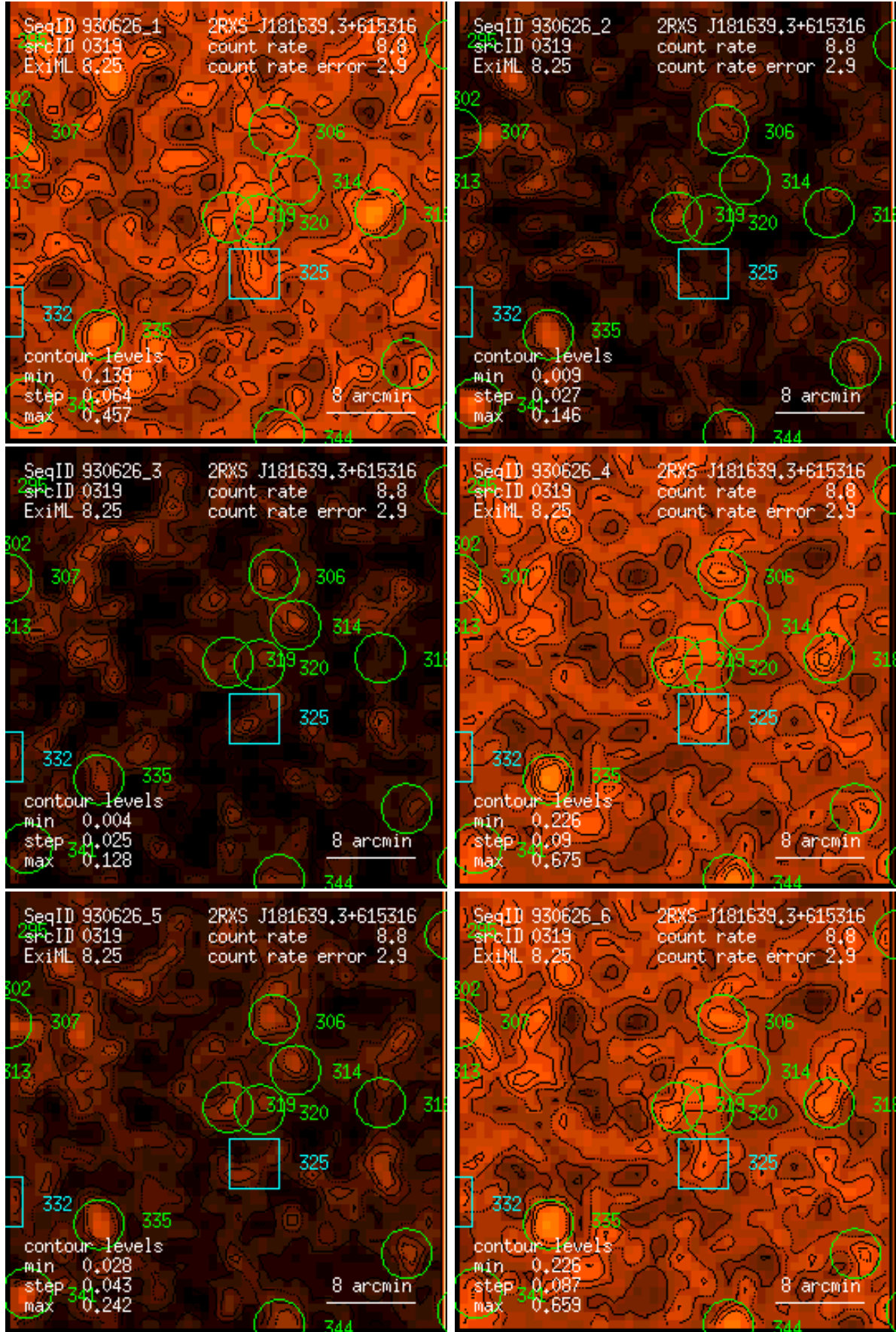
Figure 319: RASS 930626: detection 0319: band rate images, Gaussian filter: (1) PSPC channels 11 – 41, (2) 52 – 90, (3) 91 – 201, (4) 11 – 235, (5) 52 – 201, (6) 11 – 201. Broad band rates in counts/ks. Band rate contour levels in counts/ks/arcmin 2 .
