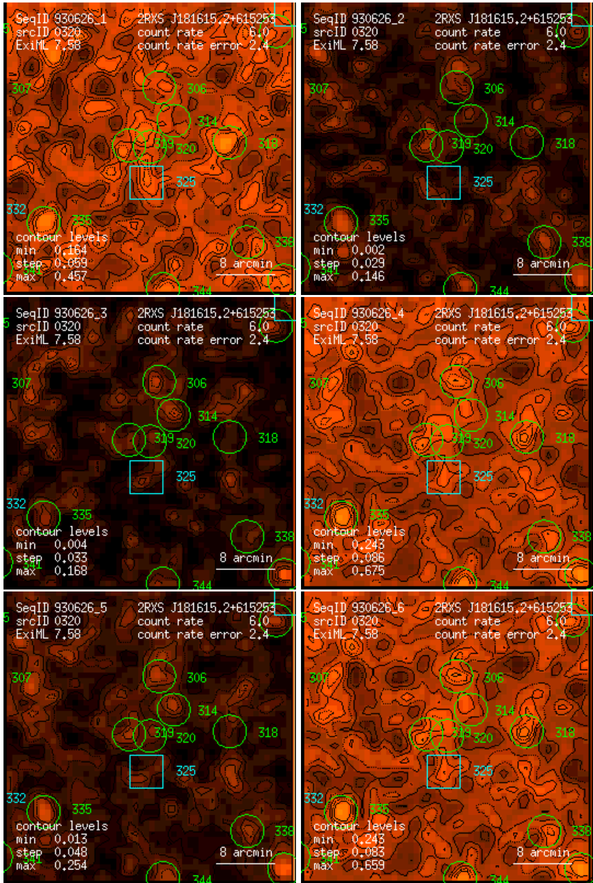
Figure 320: RASS 930626: detection 0320: band rate images, Gaussian filter: (1) PSPC channels 11 – 41, (2) 52 – 90, (3) 91 – 201, (4) 11 – 235, (5) 52 – 201, (6) 11 – 201. Broad band rates in counts/ks. Band rate contour levels in counts/ks/arcmin 2 .
