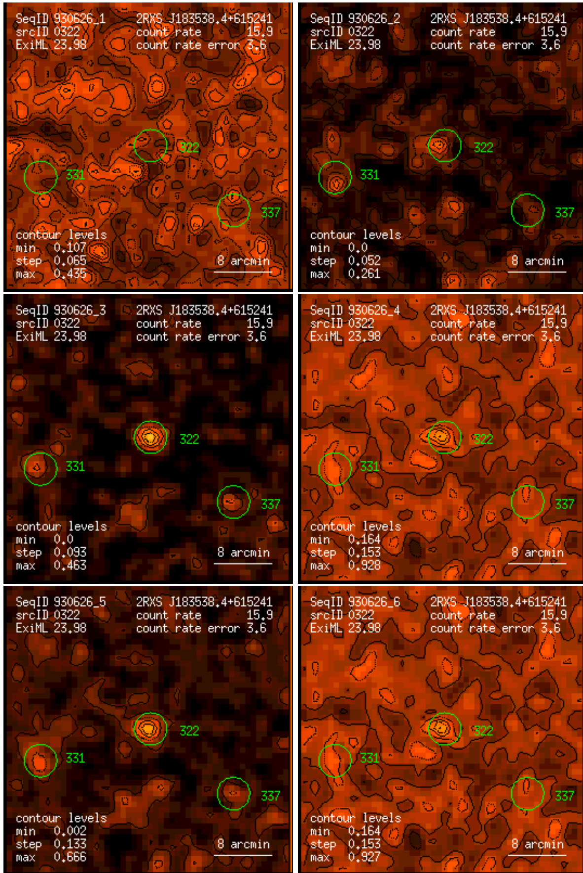
Figure 322: RASS 930626: detection 0322: band rate images, Gaussian filter: (1) PSPC channels 11 – 41, (2) 52 – 90, (3) 91 – 201, (4) 11 – 235, (5) 52 – 201, (6) 11 – 201. Broad band rates in counts/ks. Band rate contour levels in counts/ks/arcmin 2 .
