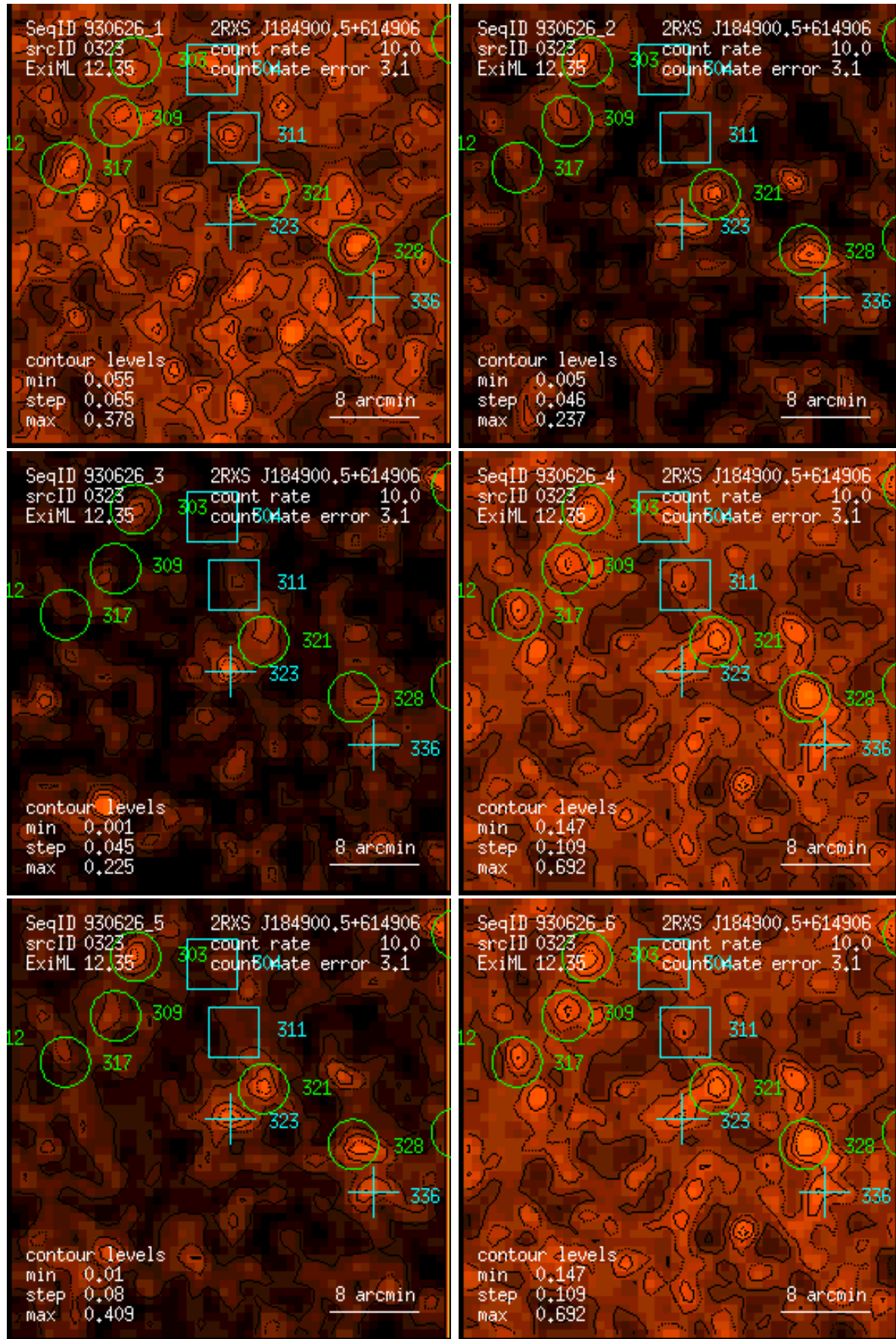
Figure 323: RASS 930626: detection 0323: band rate images, Gaussian filter: (1) PSPC channels 11 – 41, (2) 52 – 90, (3) 91 – 201, (4) 11 – 235, (5) 52 – 201, (6) 11 – 201. Broad band rates in counts/ks. Band rate contour levels in counts/ks/arcmin 2 .
