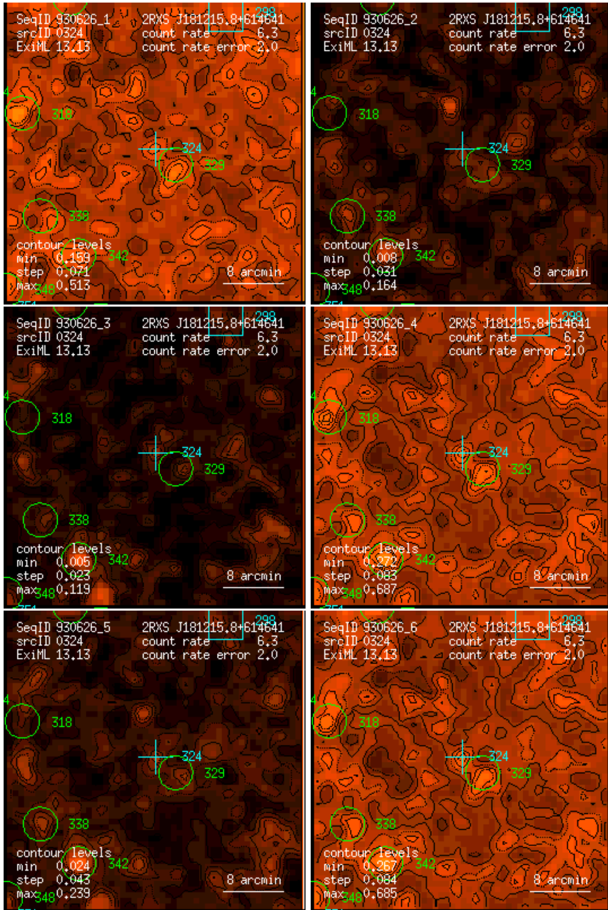
Figure 324: RASS 930626: detection 0324: band rate images, Gaussian filter: (1) PSPC channels 11 – 41, (2) 52 – 90, (3) 91 – 201, (4) 11 – 235, (5) 52 – 201, (6) 11 – 201. Broad band rates in counts/ks. Band rate contour levels in counts/ks/arcmin 2 .
