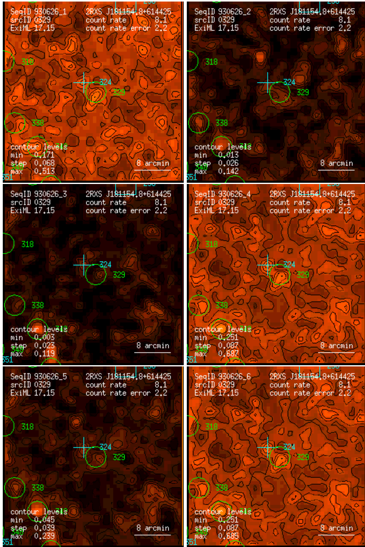
Figure 329: RASS 930626: detection 0329: band rate images, Gaussian filter: (1) PSPC channels 11 – 41, (2) 52 – 90, (3) 91 – 201, (4) 11 – 235, (5) 52 – 201, (6) 11 – 201. Broad band rates in counts/ks. Band rate contour levels in counts/ks/arcmin 2 .
