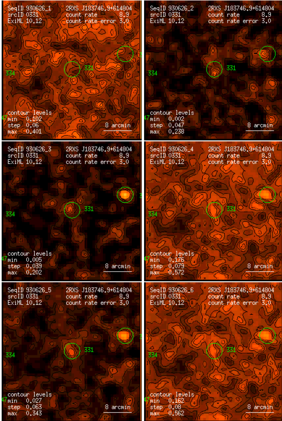
Figure 331: RASS 930626: detection 0331: band rate images, Gaussian filter: (1) PSPC channels 11 – 41, (2) 52 – 90, (3) 91 – 201, (4) 11 – 235, (5) 52 – 201, (6) 11 – 201. Broad band rates in counts/ks. Band rate contour levels in counts/ks/arcmin 2 .
