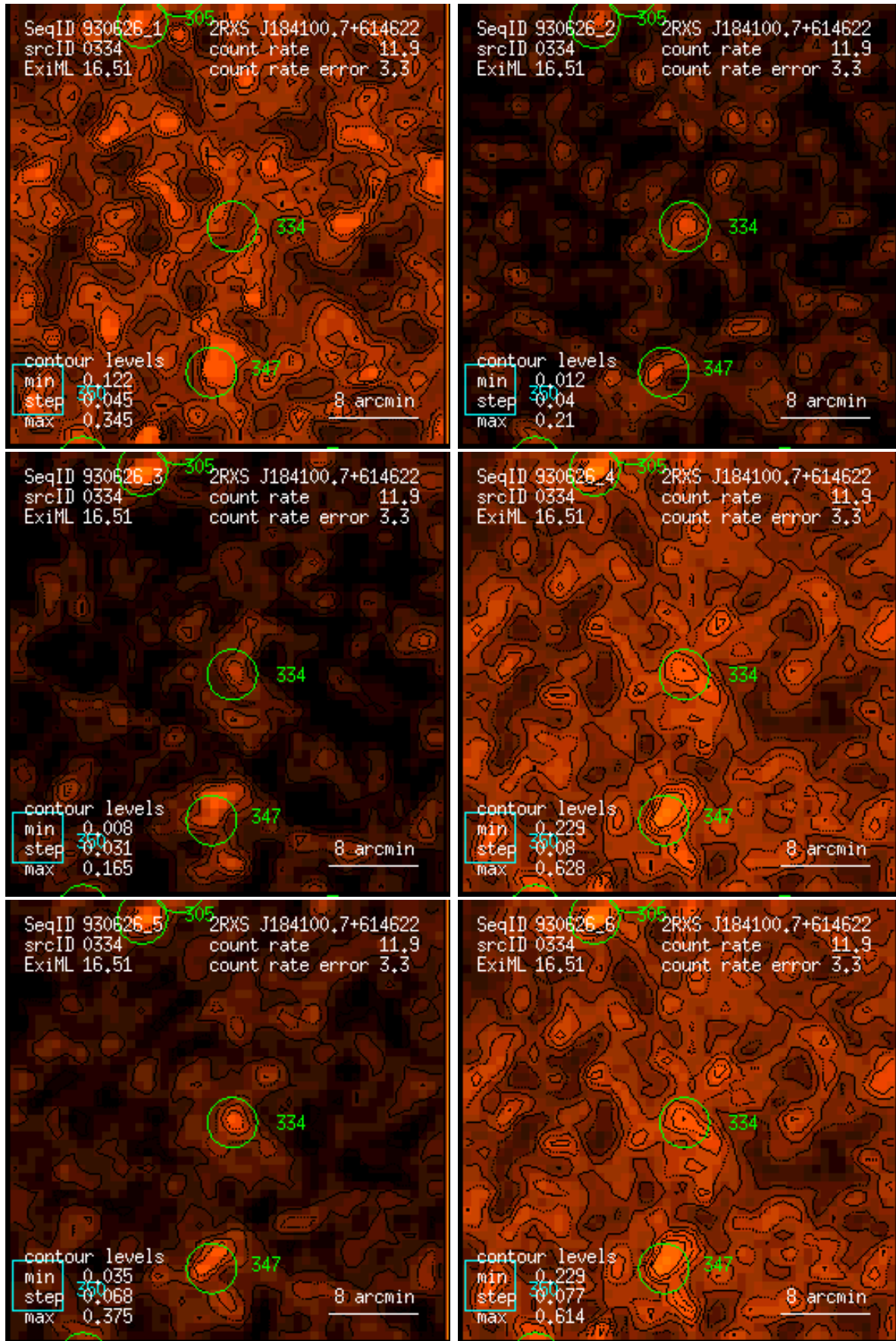
Figure 334: RASS 930626: detection 0334: band rate images, Gaussian filter: (1) PSPC channels 11 – 41, (2) 52 – 90, (3) 91 – 201, (4) 11 – 235, (5) 52 – 201, (6) 11 – 201. Broad band rates in counts/ks. Band rate contour levels in counts/ks/arcmin 2 .
