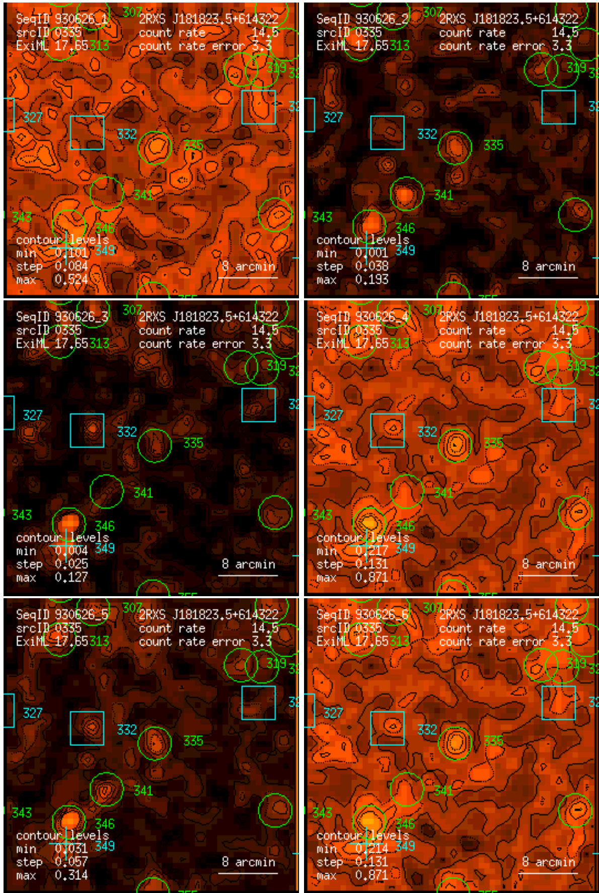
Figure 335: RASS 930626: detection 0335: band rate images, Gaussian filter: (1) PSPC channels 11 – 41, (2) 52 – 90, (3) 91 – 201, (4) 11 – 235, (5) 52 – 201, (6) 11 – 201. Broad band rates in counts/ks. Band rate contour levels in counts/ks/arcmin 2 .
