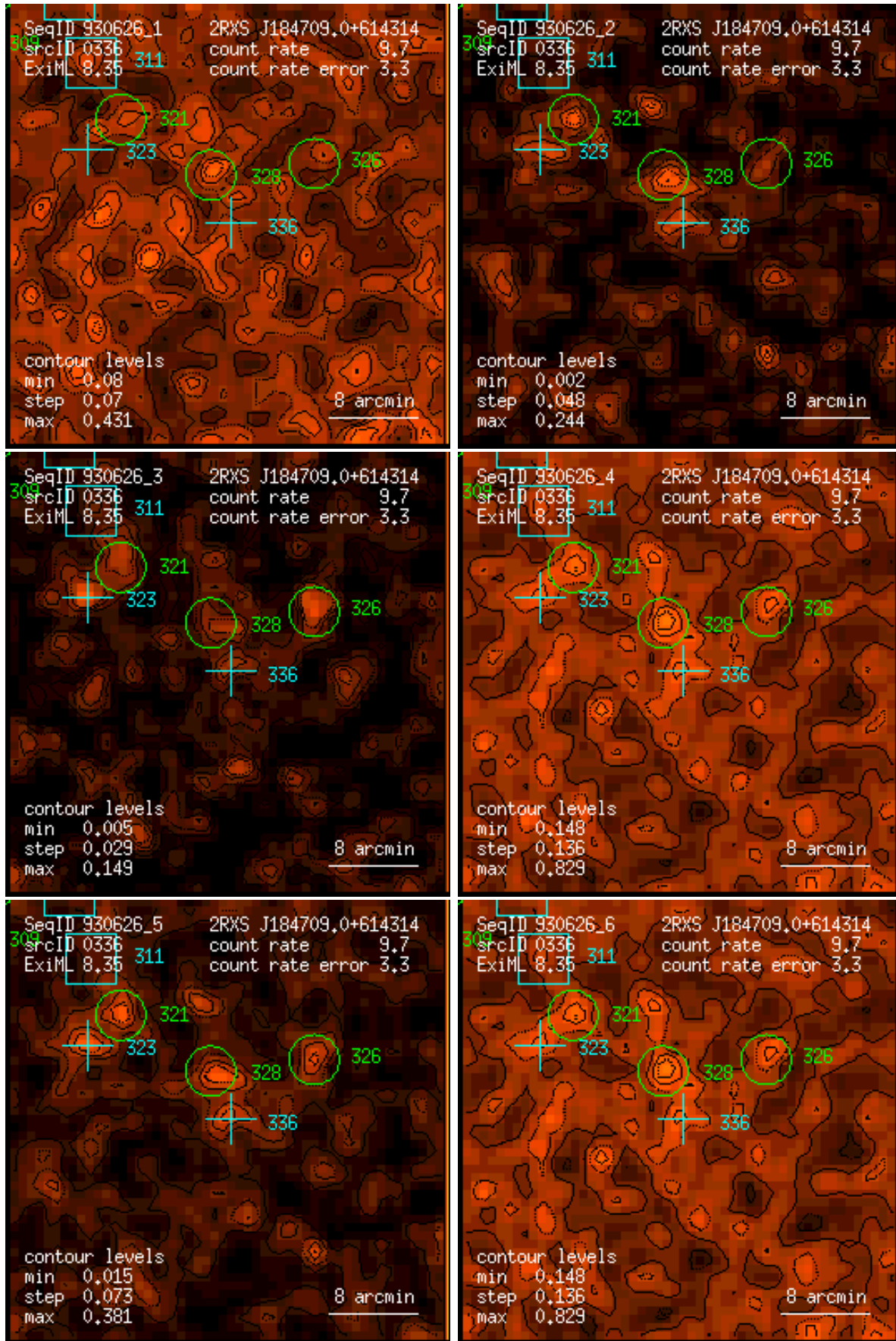
Figure 336: RASS 930626: detection 0336: band rate images, Gaussian filter: (1) PSPC channels 11 – 41, (2) 52 – 90, (3) 91 – 201, (4) 11 – 235, (5) 52 – 201, (6) 11 – 201. Broad band rates in counts/ks. Band rate contour levels in counts/ks/arcmin 2 .
