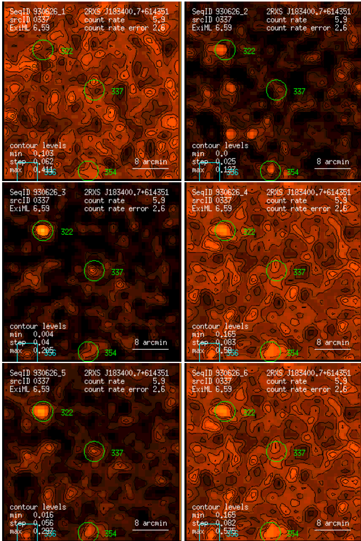
Figure 337: RASS 930626: detection 0337: band rate images, Gaussian filter: (1) PSPC channels 11 – 41, (2) 52 – 90, (3) 91 – 201, (4) 11 – 235, (5) 52 – 201, (6) 11 – 201. Broad band rates in counts/ks. Band rate contour levels in counts/ks/arcmin 2 .
