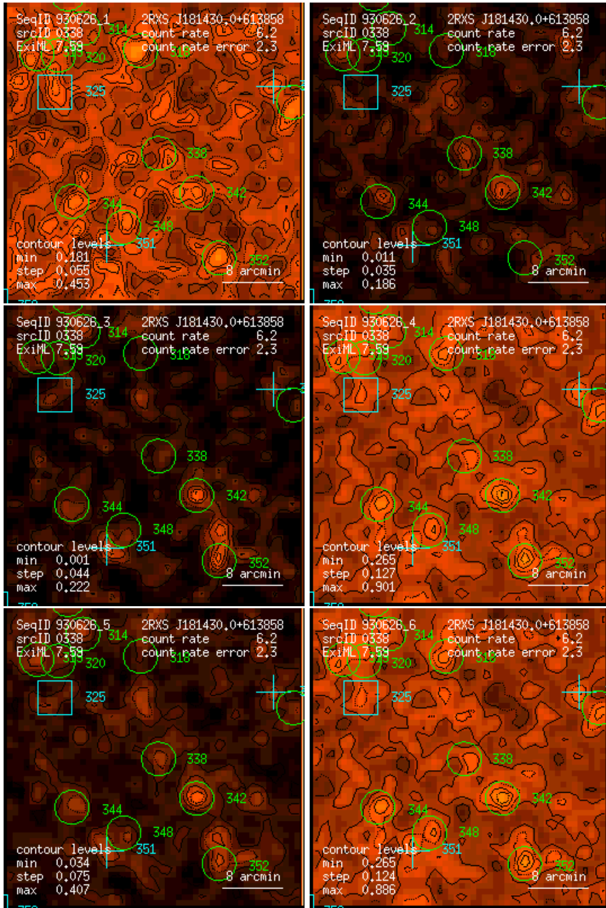
Figure 338: RASS 930626: detection 0338: band rate images, Gaussian filter: (1) PSPC channels 11 – 41, (2) 52 – 90, (3) 91 – 201, (4) 11 – 235, (5) 52 – 201, (6) 11 – 201. Broad band rates in counts/ks. Band rate contour levels in counts/ks/arcmin 2 .
