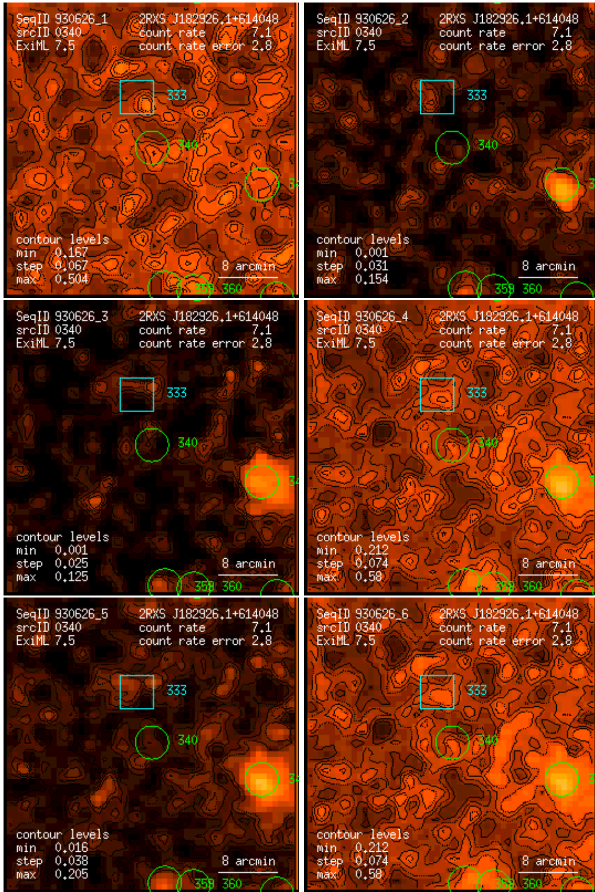
Figure 340: RASS 930626: detection 0340: band rate images, Gaussian filter: (1) PSPC channels 11 – 41, (2) 52 – 90, (3) 91 – 201, (4) 11 – 235, (5) 52 – 201, (6) 11 – 201. Broad band rates in counts/ks. Band rate contour levels in counts/ks/arcmin 2 .
