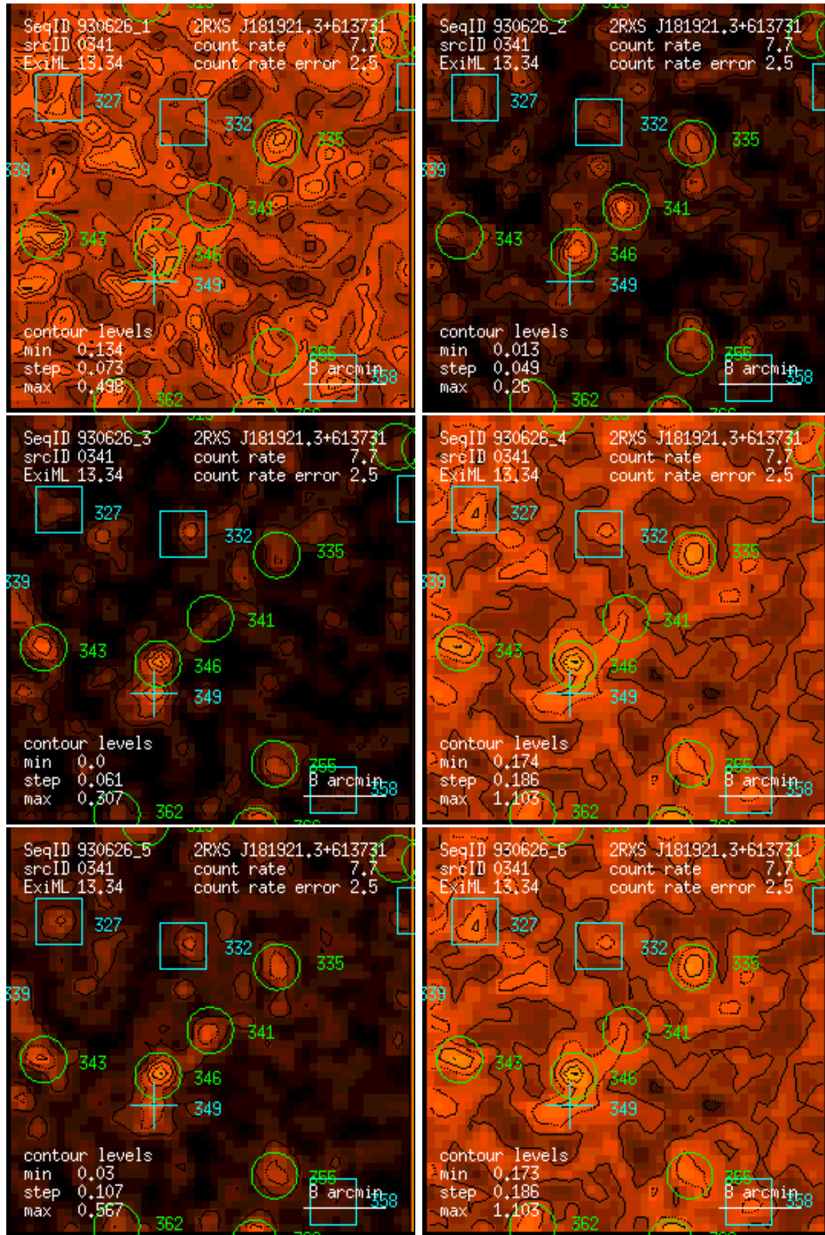
Figure 341: RASS 930626: detection 0341: band rate images, Gaussian filter: (1) PSPC channels 11 – 41, (2) 52 – 90, (3) 91 – 201, (4) 11 – 235, (5) 52 – 201, (6) 11 – 201. Broad band rates in counts/ks. Band rate contour levels in counts/ks/arcmin 2 .
