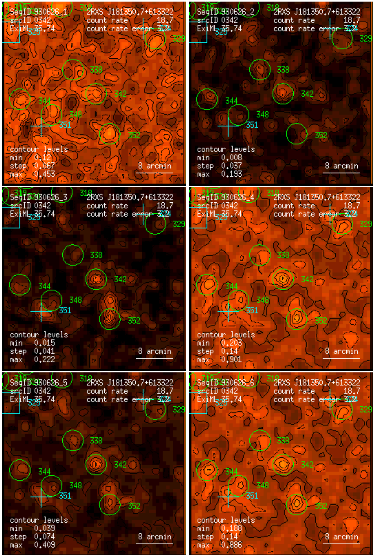
Figure 342: RASS 930626: detection 0342: band rate images, Gaussian filter: (1) PSPC channels 11 – 41, (2) 52 – 90, (3) 91 – 201, (4) 11 – 235, (5) 52 – 201, (6) 11 – 201. Broad band rates in counts/ks. Band rate contour levels in counts/ks/arcmin 2 .
