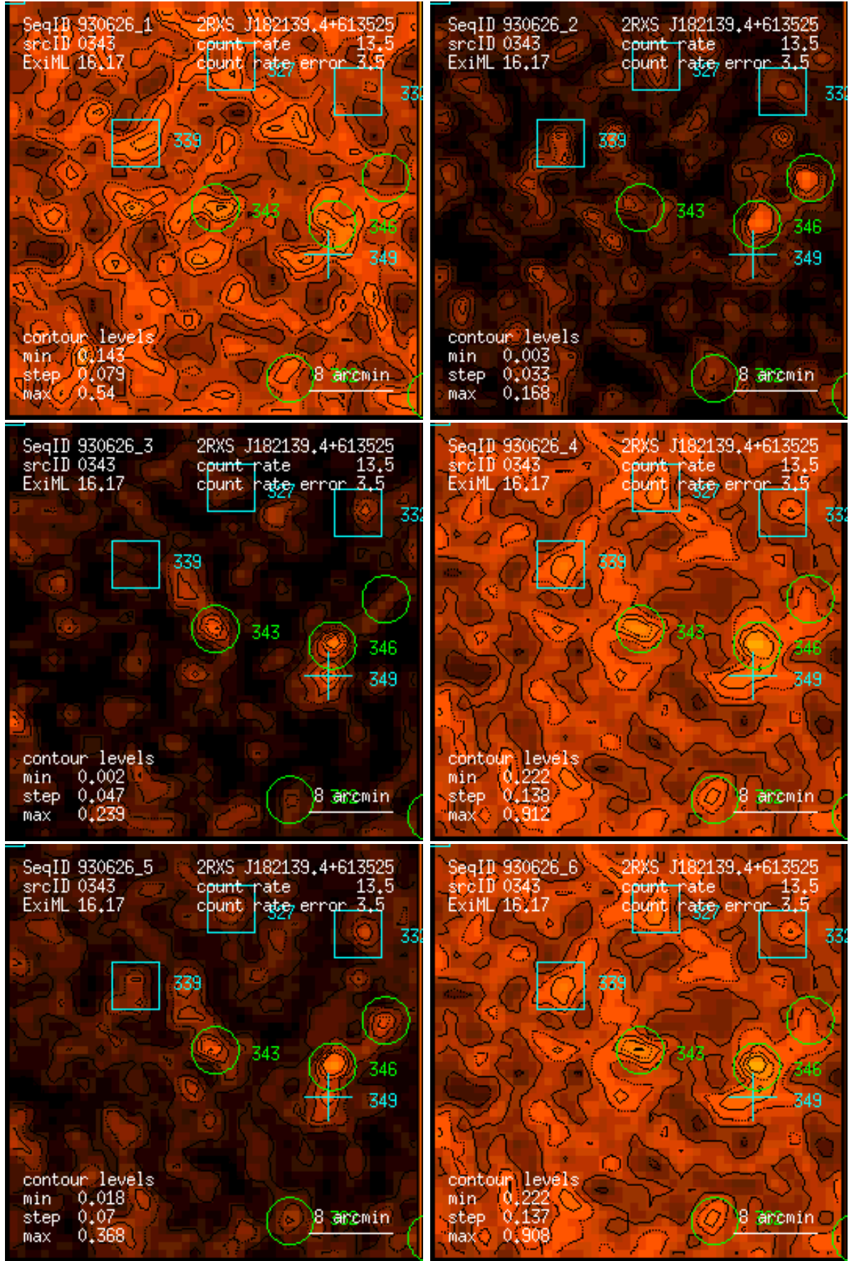
Figure 343: RASS 930626: detection 0343: band rate images, Gaussian filter: (1) PSPC channels 11 – 41, (2) 52 – 90, (3) 91 – 201, (4) 11 – 235, (5) 52 – 201, (6) 11 – 201. Broad band rates in counts/ks. Band rate contour levels in counts/ks/arcmin 2 .
