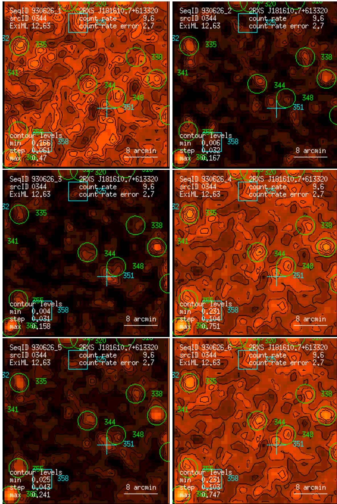
Figure 344: RASS 930626: detection 0344: band rate images, Gaussian filter: (1) PSPC channels 11 – 41, (2) 52 – 90, (3) 91 – 201, (4) 11 – 235, (5) 52 – 201, (6) 11 – 201. Broad band rates in counts/ks. Band rate contour levels in counts/ks/arcmin 2 .
