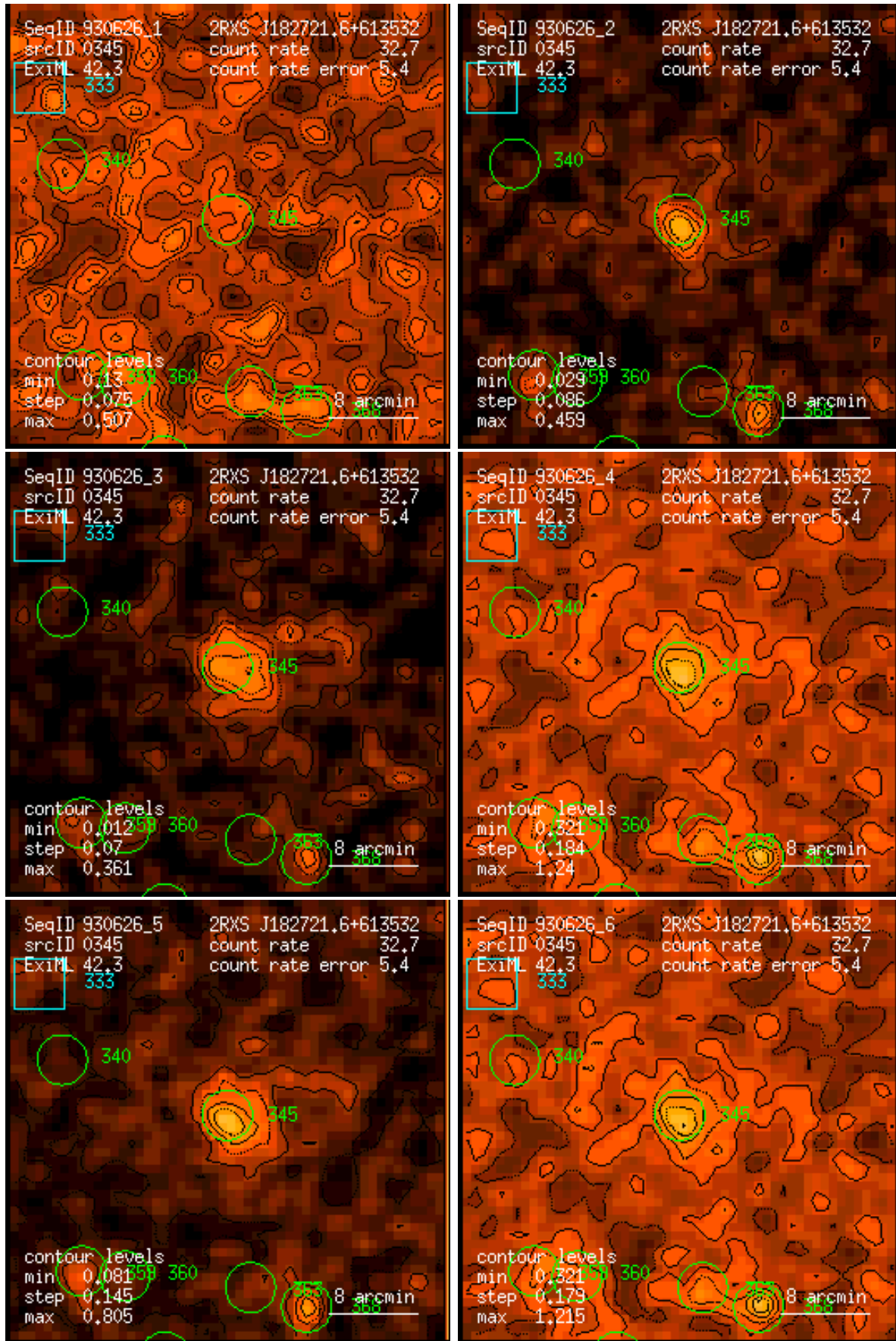
Figure 345: RASS 930626: detection 0345: band rate images, Gaussian filter: (1) PSPC channels 11 – 41, (2) 52 – 90, (3) 91 – 201, (4) 11 – 235, (5) 52 – 201, (6) 11 – 201. Broad band rates in counts/ks. Band rate contour levels in counts/ks/arcmin 2 .
