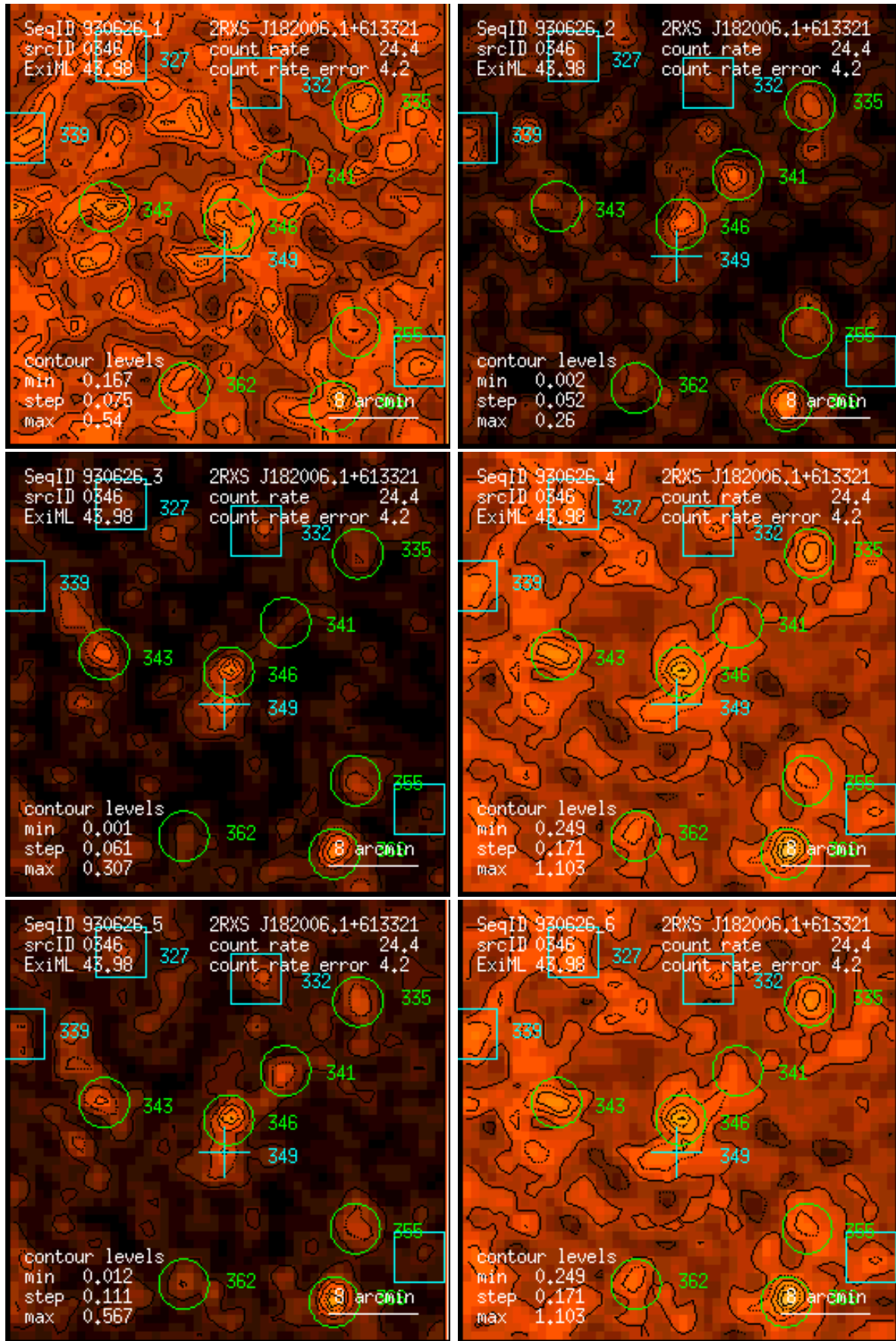
Figure 346: RASS 930626: detection 0346: band rate images, Gaussian filter: (1) PSPC channels 11 – 41, (2) 52 – 90, (3) 91 – 201, (4) 11 – 235, (5) 52 – 201, (6) 11 – 201. Broad band rates in counts/ks. Band rate contour levels in counts/ks/arcmin 2 .
