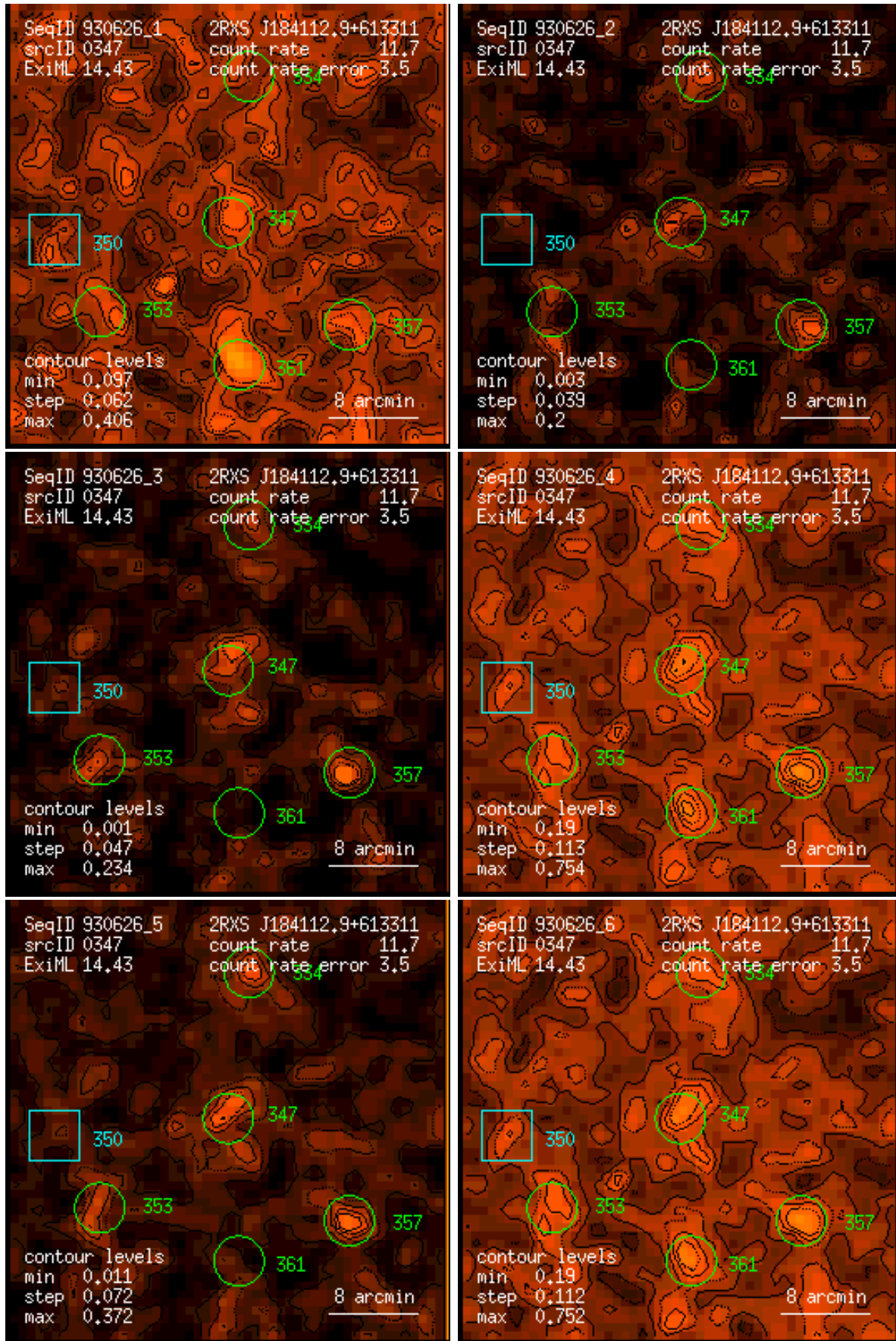
Figure 347: RASS 930626: detection 0347: band rate images, Gaussian filter: (1) PSPC channels 11 – 41, (2) 52 – 90, (3) 91 – 201, (4) 11 – 235, (5) 52 – 201, (6) 11 – 201. Broad band rates in counts/ks. Band rate contour levels in counts/ks/arcmin 2 .
