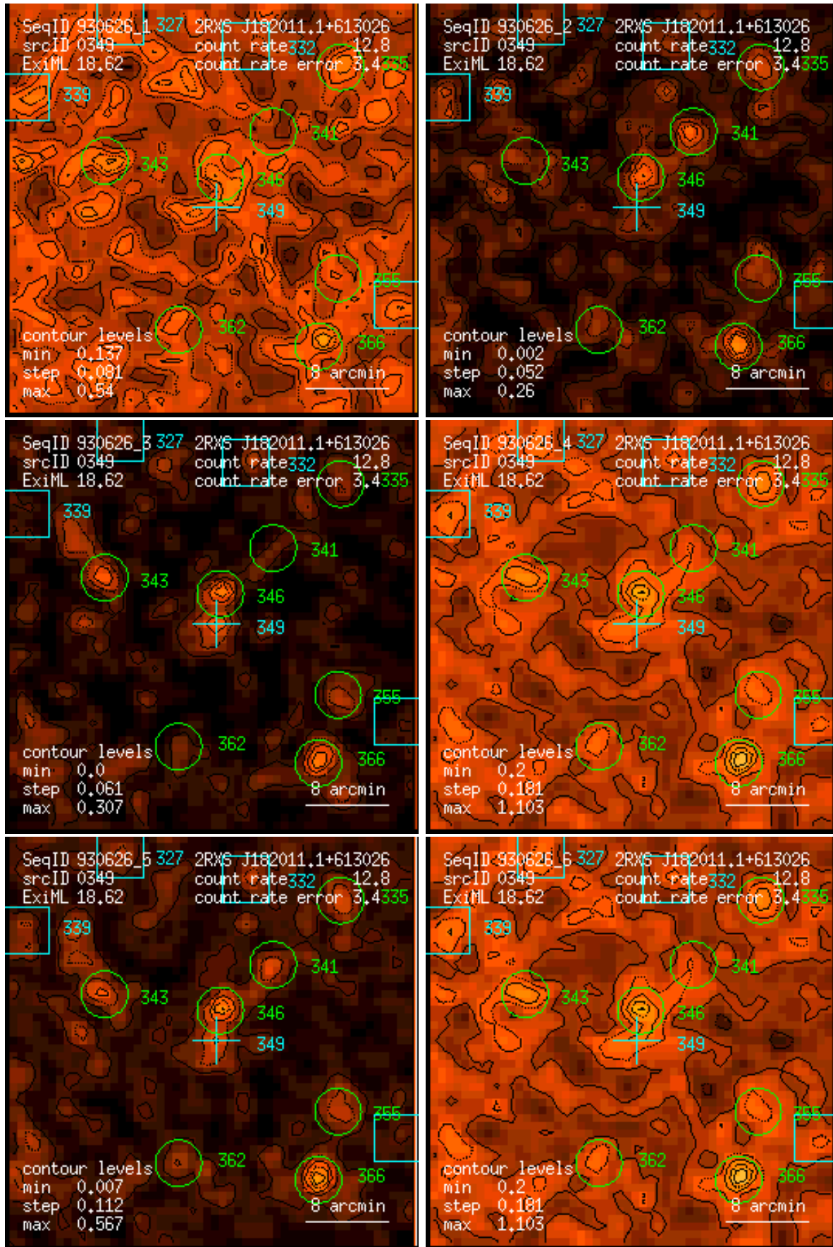
Figure 349: RASS 930626: detection 0349: band rate images, Gaussian filter: (1) PSPC channels 11 – 41, (2) 52 – 90, (3) 91 – 201, (4) 11 – 235, (5) 52 – 201, (6) 11 – 201. Broad band rates in counts/ks. Band rate contour levels in counts/ks/arcmin 2 .
