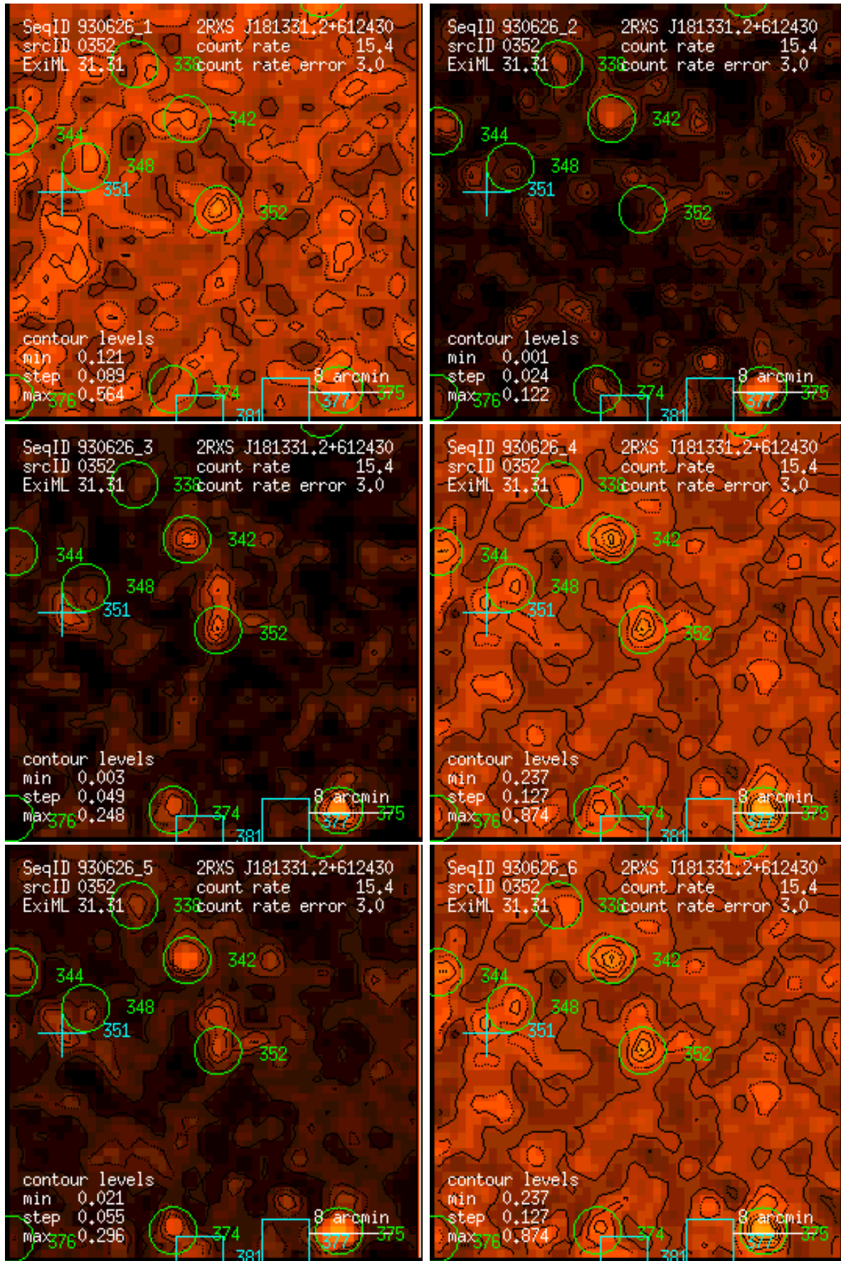
Figure 352: RASS 930626: detection 0352: band rate images, Gaussian filter: (1) PSPC channels 11 – 41, (2) 52 – 90, (3) 91 – 201, (4) 11 – 235, (5) 52 – 201, (6) 11 – 201. Broad band rates in counts/ks. Band rate contour levels in counts/ks/arcmin 2 .
