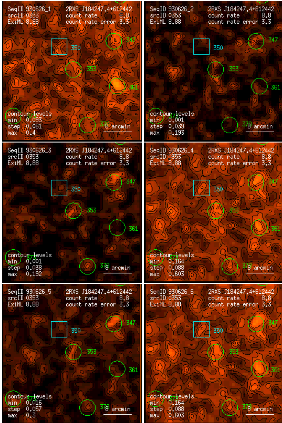
Figure 353: RASS 930626: detection 0353: band rate images, Gaussian filter: (1) PSPC channels 11 – 41, (2) 52 – 90, (3) 91 – 201, (4) 11 – 235, (5) 52 – 201, (6) 11 – 201. Broad band rates in counts/ks. Band rate contour levels in counts/ks/arcmin 2 .
