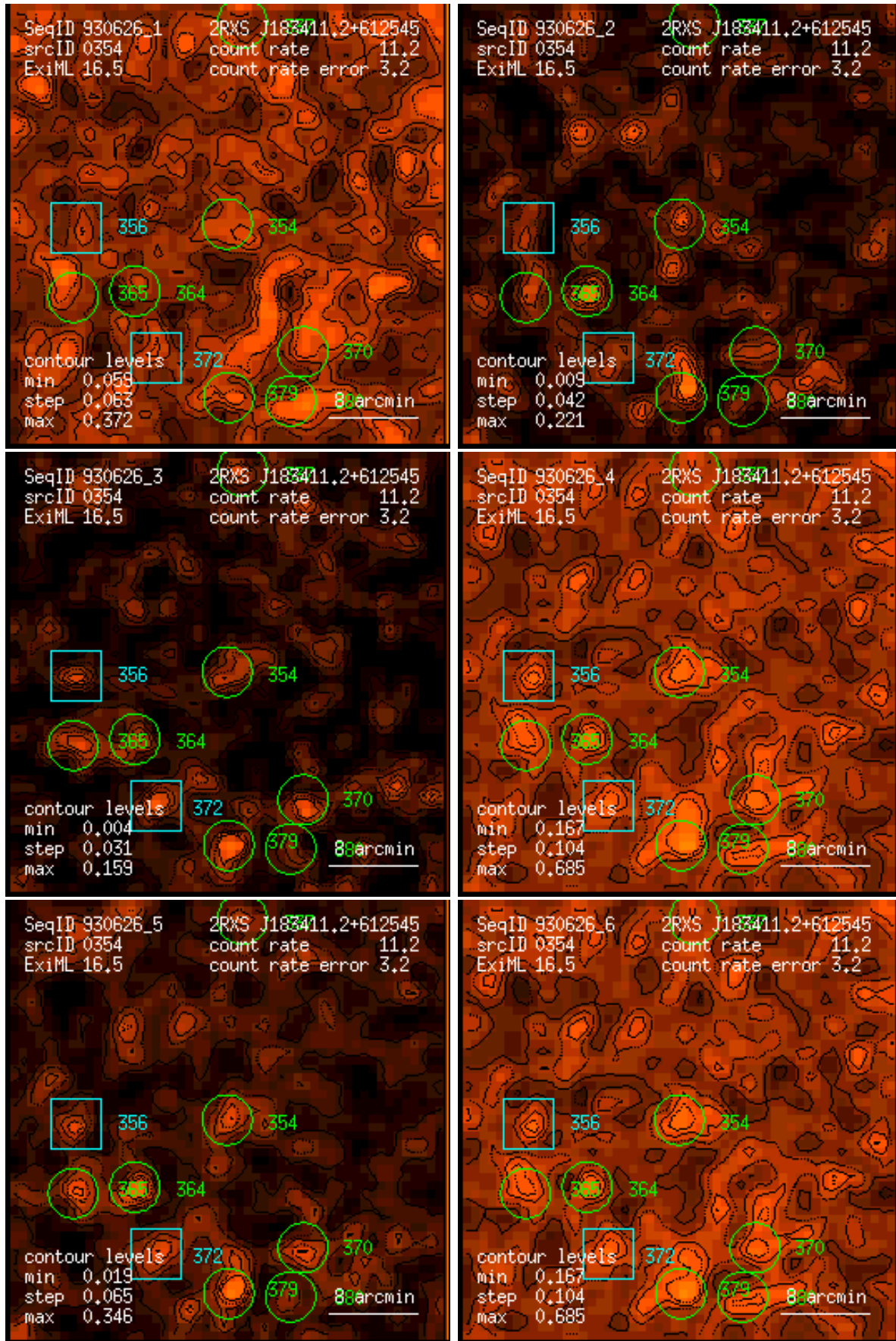
Figure 354: RASS 930626: detection 0354: band rate images, Gaussian filter: (1) PSPC channels 11 – 41, (2) 52 – 90, (3) 91 – 201, (4) 11 – 235, (5) 52 – 201, (6) 11 – 201. Broad band rates in counts/ks. Band rate contour levels in counts/ks/arcmin 2 .
