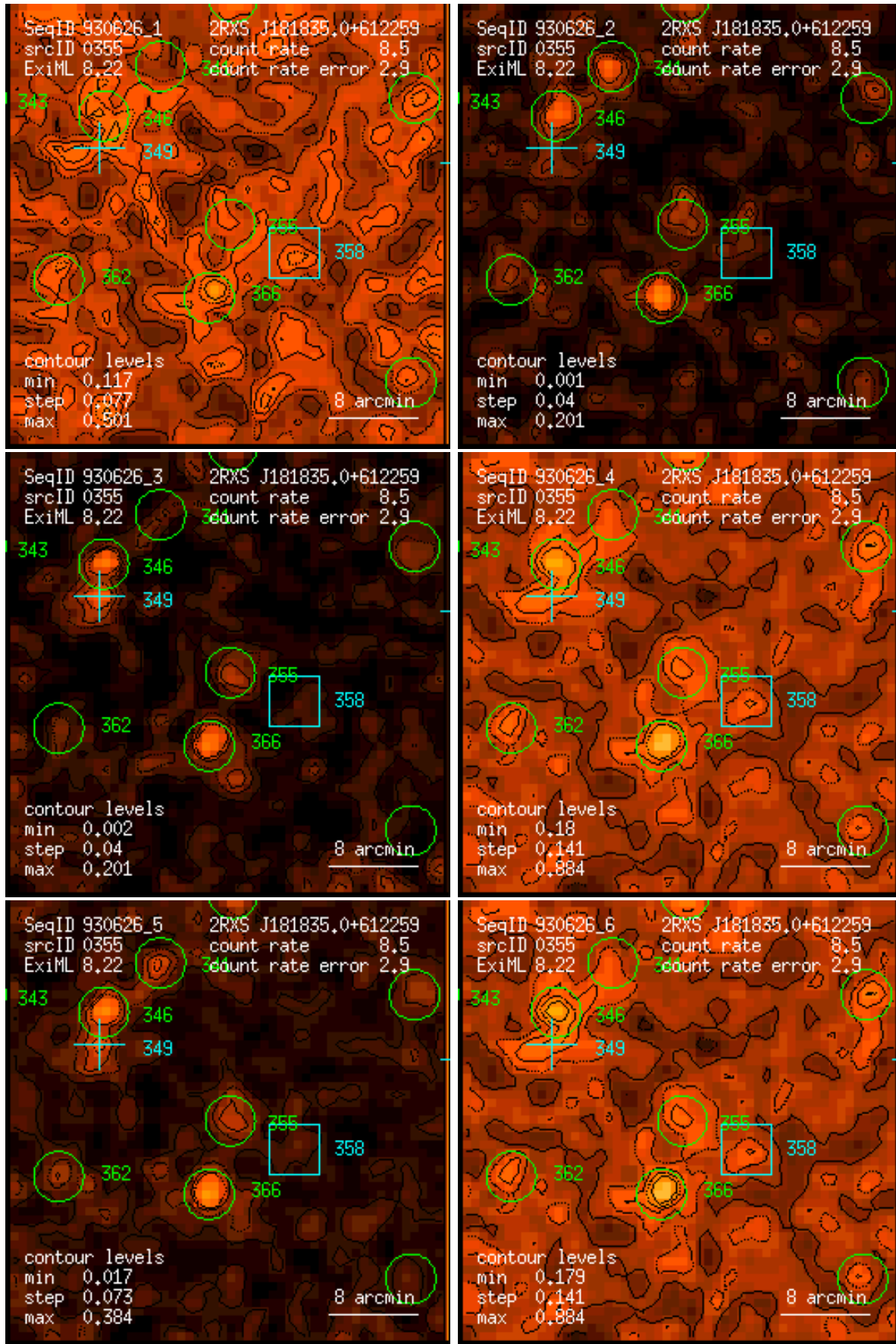
Figure 355: RASS 930626: detection 0355: band rate images, Gaussian filter: (1) PSPC channels 11 – 41, (2) 52 – 90, (3) 91 – 201, (4) 11 – 235, (5) 52 – 201, (6) 11 – 201. Broad band rates in counts/ks. Band rate contour levels in counts/ks/arcmin 2 .
