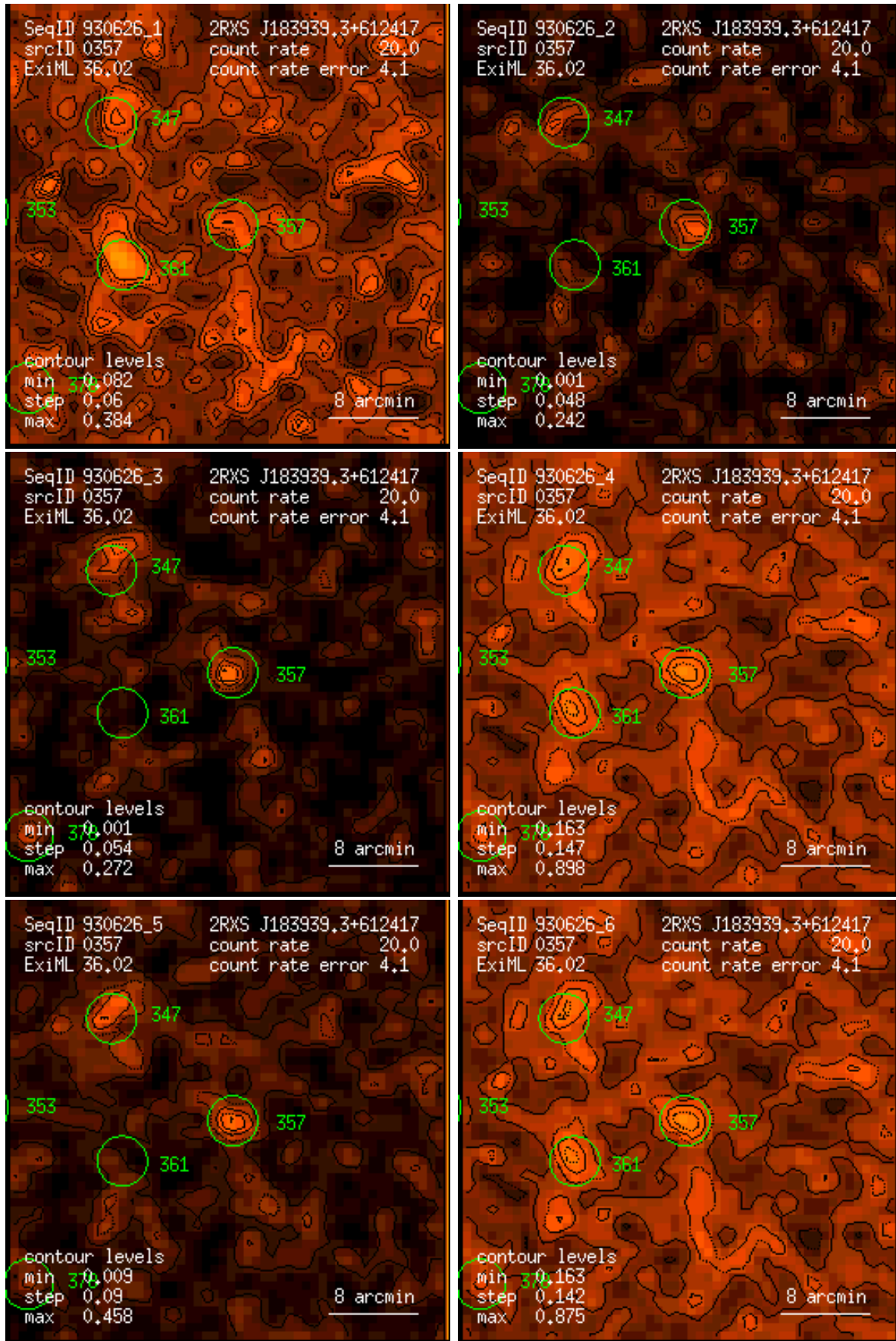
Figure 357: RASS 930626: detection 0357: band rate images, Gaussian filter: (1) PSPC channels 11 – 41, (2) 52 – 90, (3) 91 – 201, (4) 11 – 235, (5) 52 – 201, (6) 11 – 201. Broad band rates in counts/ks. Band rate contour levels in counts/ks/arcmin 2 .
