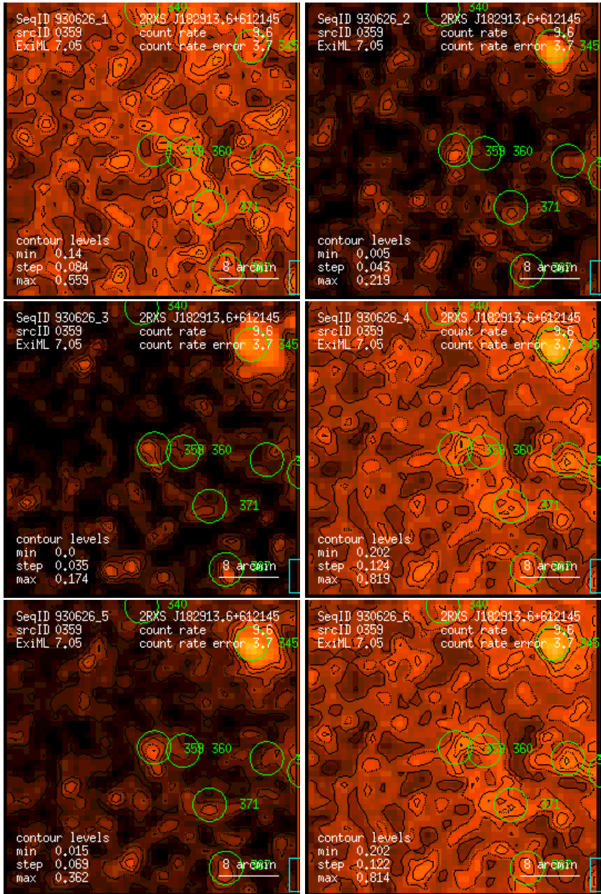
Figure 359: RASS 930626: detection 0359: band rate images, Gaussian filter: (1) PSPC channels 11 – 41, (2) 52 – 90, (3) 91 – 201, (4) 11 – 235, (5) 52 – 201, (6) 11 – 201. Broad band rates in counts/ks. Band rate contour levels in counts/ks/arcmin 2 .
