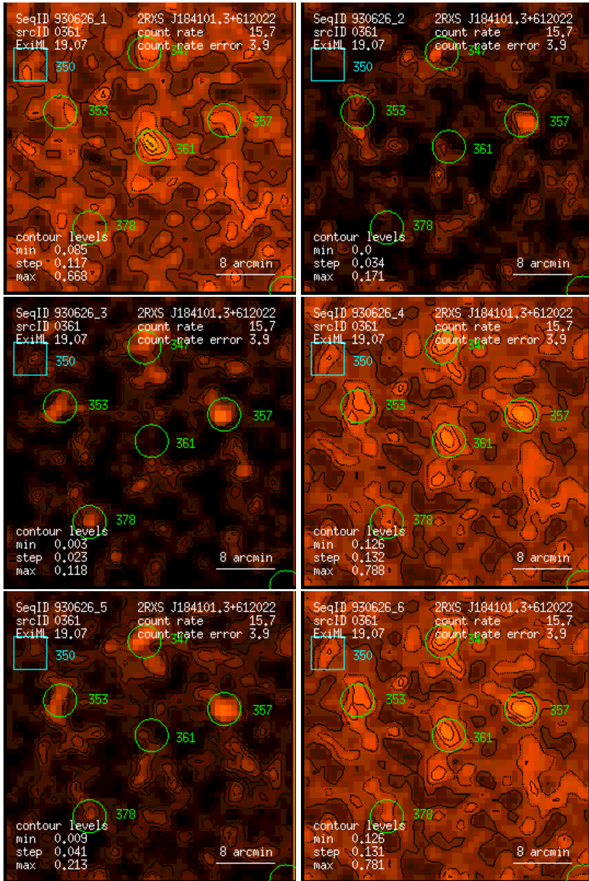
Figure 361: RASS 930626: detection 0361: band rate images, Gaussian filter: (1) PSPC channels 11 – 41, (2) 52 – 90, (3) 91 – 201, (4) 11 – 235, (5) 52 – 201, (6) 11 – 201. Broad band rates in counts/ks. Band rate contour levels in counts/ks/arcmin 2 .
