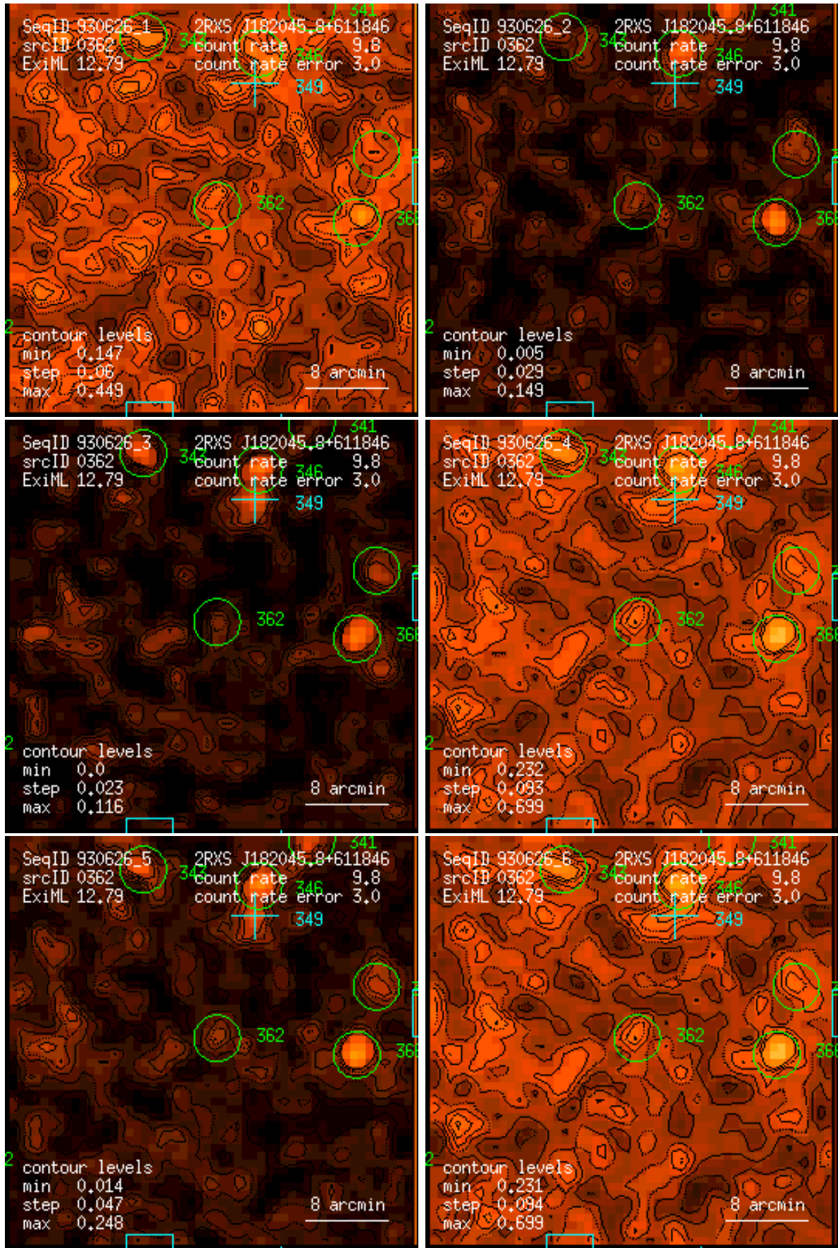
Figure 362: RASS 930626: detection 0362: band rate images, Gaussian filter: (1) PSPC channels 11 – 41, (2) 52 – 90, (3) 91 – 201, (4) 11 – 235, (5) 52 – 201, (6) 11 – 201. Broad band rates in counts/ks. Band rate contour levels in counts/ks/arcmin 2 .
