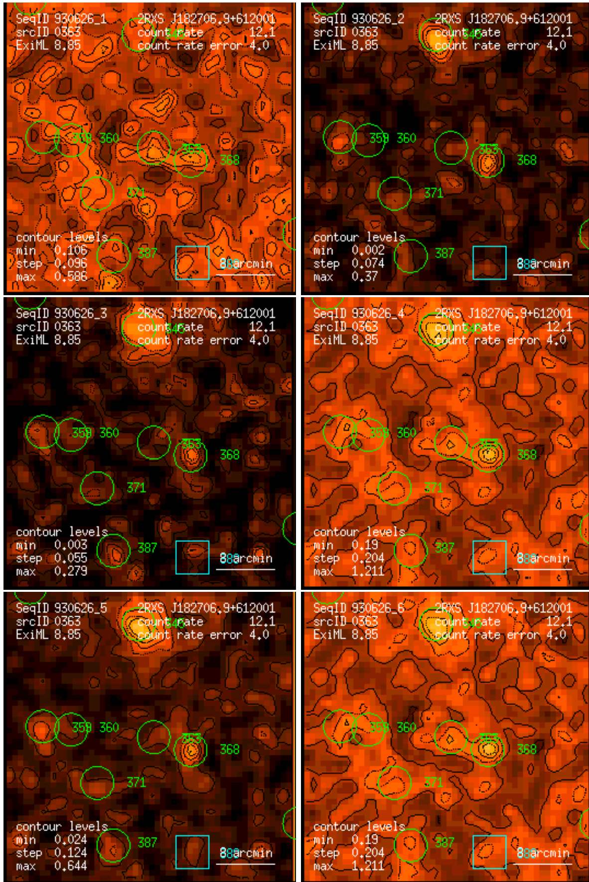
Figure 363: RASS 930626: detection 0363: band rate images, Gaussian filter: (1) PSPC channels 11 – 41, (2) 52 – 90, (3) 91 – 201, (4) 11 – 235, (5) 52 – 201, (6) 11 – 201. Broad band rates in counts/ks. Band rate contour levels in counts/ks/arcmin 2 .
