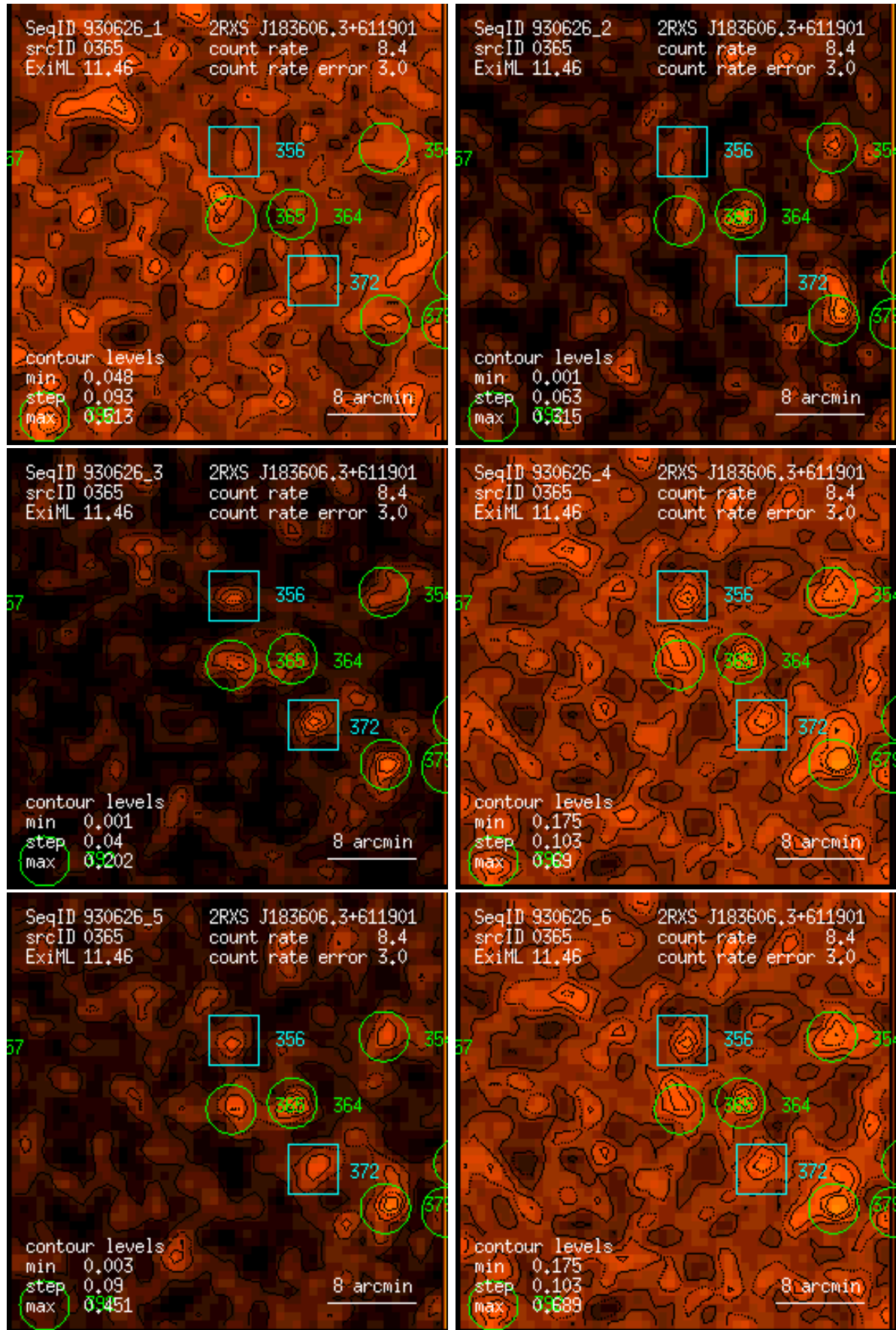
Figure 365: RASS 930626: detection 0365: band rate images, Gaussian filter: (1) PSPC channels 11 – 41, (2) 52 – 90, (3) 91 – 201, (4) 11 – 235, (5) 52 – 201, (6) 11 – 201. Broad band rates in counts/ks. Band rate contour levels in counts/ks/arcmin 2 .
