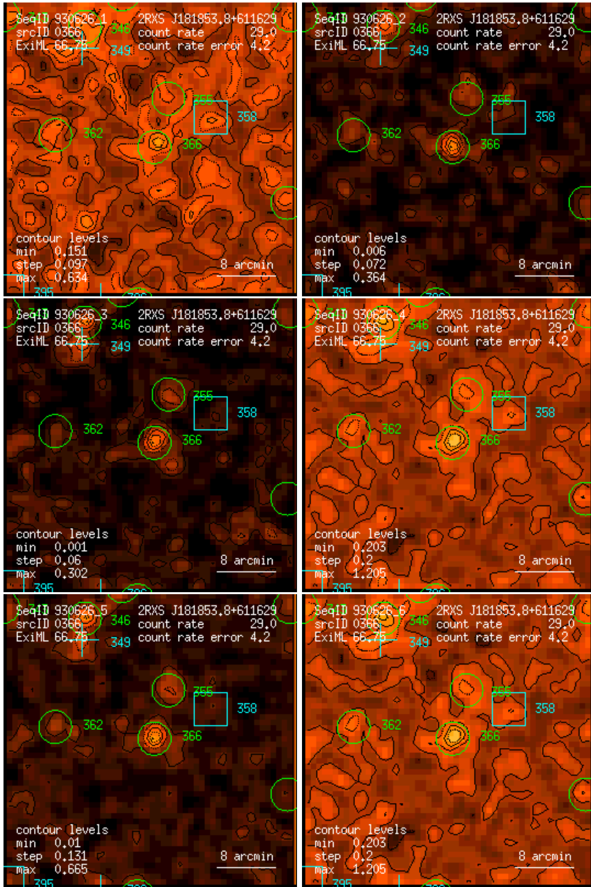
Figure 366: RASS 930626: detection 0366: band rate images, Gaussian filter: (1) PSPC channels 11 – 41, (2) 52 – 90, (3) 91 – 201, (4) 11 – 235, (5) 52 – 201, (6) 11 – 201. Broad band rates in counts/ks. Band rate contour levels in counts/ks/arcmin 2 .
