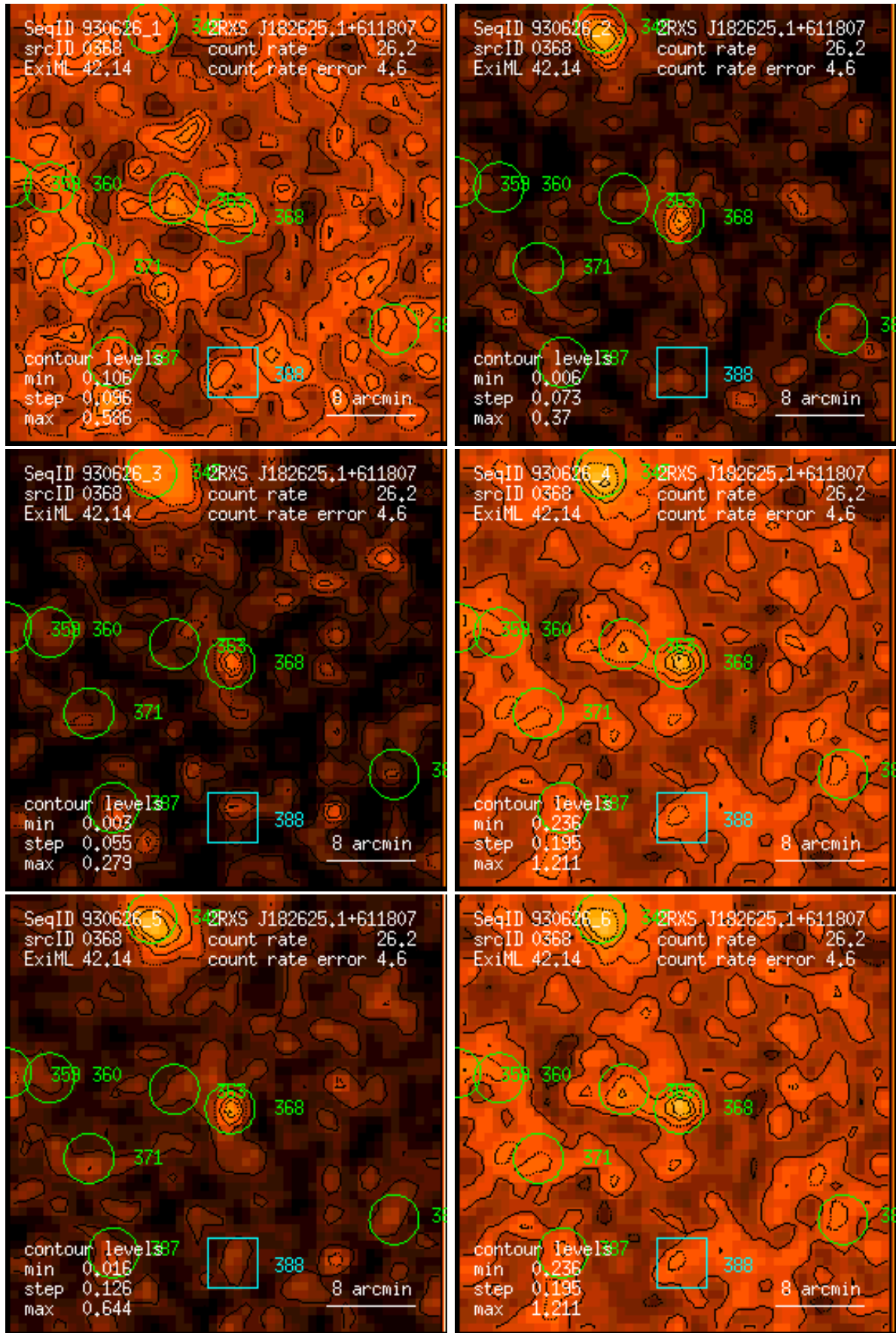
Figure 368: RASS 930626: detection 0368: band rate images, Gaussian filter: (1) PSPC channels 11 – 41, (2) 52 – 90, (3) 91 – 201, (4) 11 – 235, (5) 52 – 201, (6) 11 – 201. Broad band rates in counts/ks. Band rate contour levels in counts/ks/arcmin 2 .
