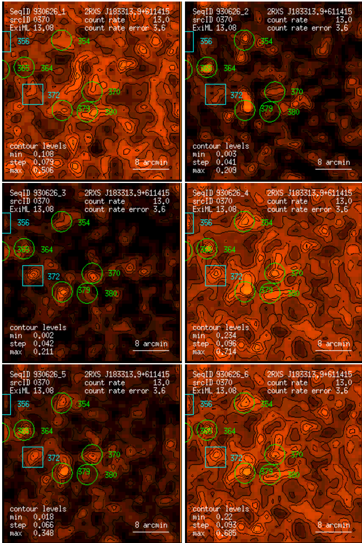
Figure 370: RASS 930626: detection 0370: band rate images, Gaussian filter: (1) PSPC channels 11 – 41, (2) 52 – 90, (3) 91 – 201, (4) 11 – 235, (5) 52 – 201, (6) 11 – 201. Broad band rates in counts/ks. Band rate contour levels in counts/ks/arcmin 2 .
