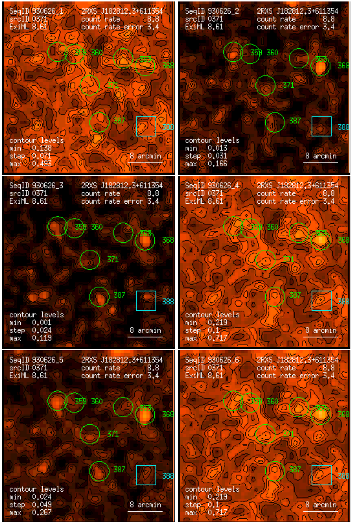
Figure 371: RASS 930626: detection 0371: band rate images, Gaussian filter: (1) PSPC channels 11 – 41, (2) 52 – 90, (3) 91 – 201, (4) 11 – 235, (5) 52 – 201, (6) 11 – 201. Broad band rates in counts/ks. Band rate contour levels in counts/ks/arcmin 2 .
