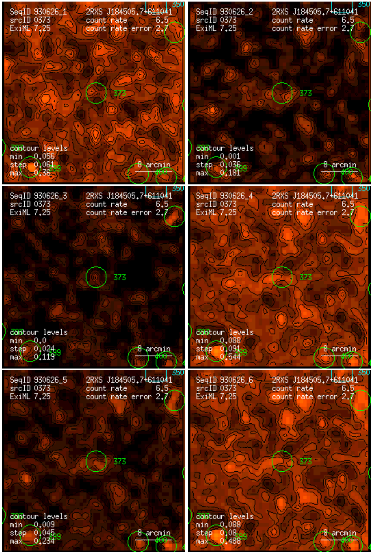
Figure 373: RASS 930626: detection 0373: band rate images, Gaussian filter: (1) PSPC channels 11 – 41, (2) 52 – 90, (3) 91 – 201, (4) 11 – 235, (5) 52 – 201, (6) 11 – 201. Broad band rates in counts/ks. Band rate contour levels in counts/ks/arcmin 2 .
