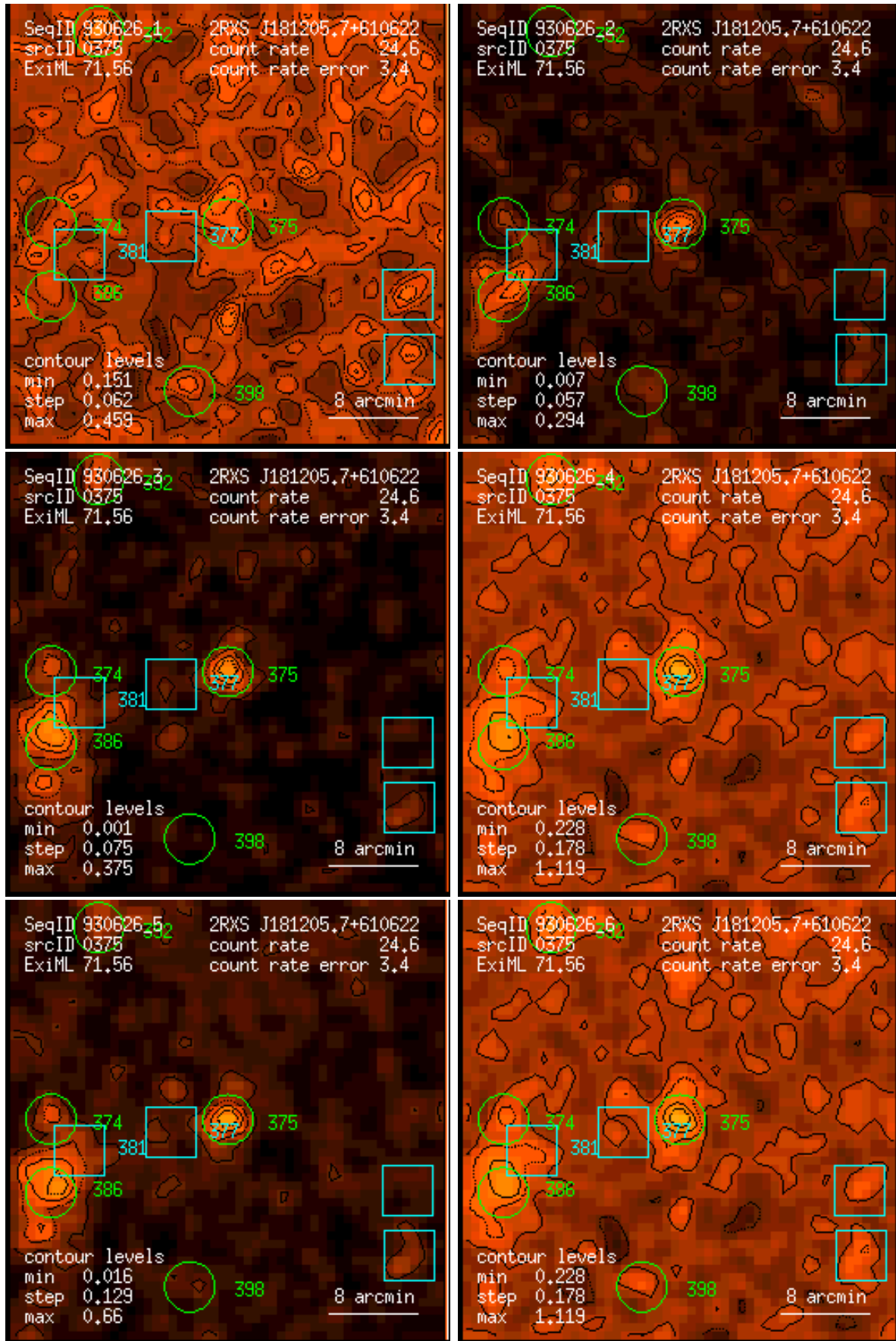
Figure 375: RASS 930626: detection 0375: band rate images, Gaussian filter: (1) PSPC channels 11 – 41, (2) 52 – 90, (3) 91 – 201, (4) 11 – 235, (5) 52 – 201, (6) 11 – 201. Broad band rates in counts/ks. Band rate contour levels in counts/ks/arcmin 2 .
