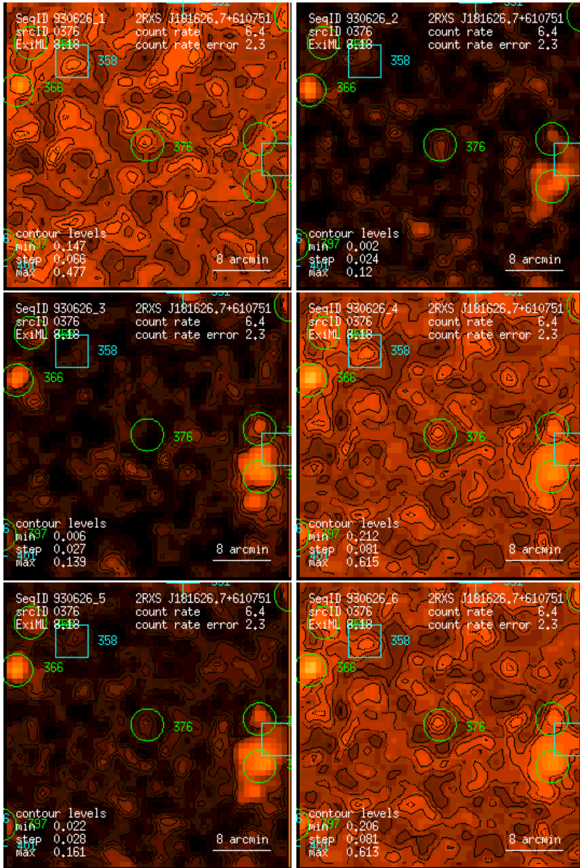
Figure 376: RASS 930626: detection 0376: band rate images, Gaussian filter: (1) PSPC channels 11 – 41, (2) 52 – 90, (3) 91 – 201, (4) 11 – 235, (5) 52 – 201, (6) 11 – 201. Broad band rates in counts/ks. Band rate contour levels in counts/ks/arcmin 2 .
