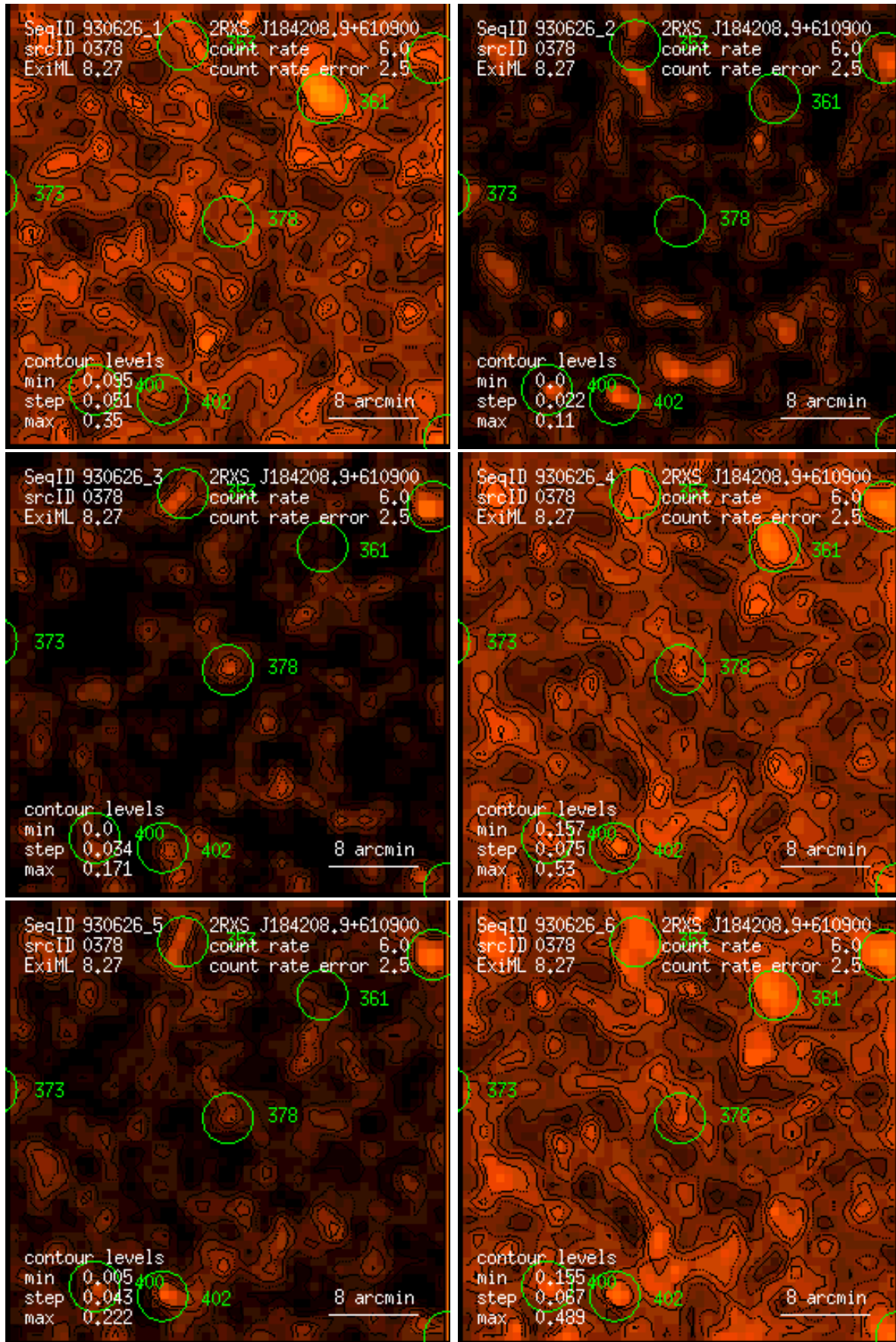
Figure 378: RASS 930626: detection 0378: band rate images, Gaussian filter: (1) PSPC channels 11 – 41, (2) 52 – 90, (3) 91 – 201, (4) 11 – 235, (5) 52 – 201, (6) 11 – 201. Broad band rates in counts/ks. Band rate contour levels in counts/ks/arcmin 2 .
